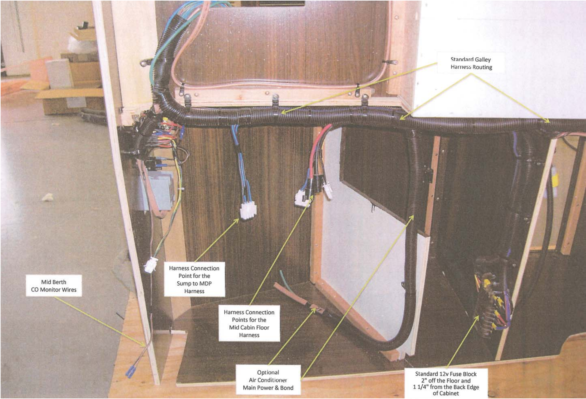
26 EXPRESS GALLEY ELECTRIC BREAKOUT 1
