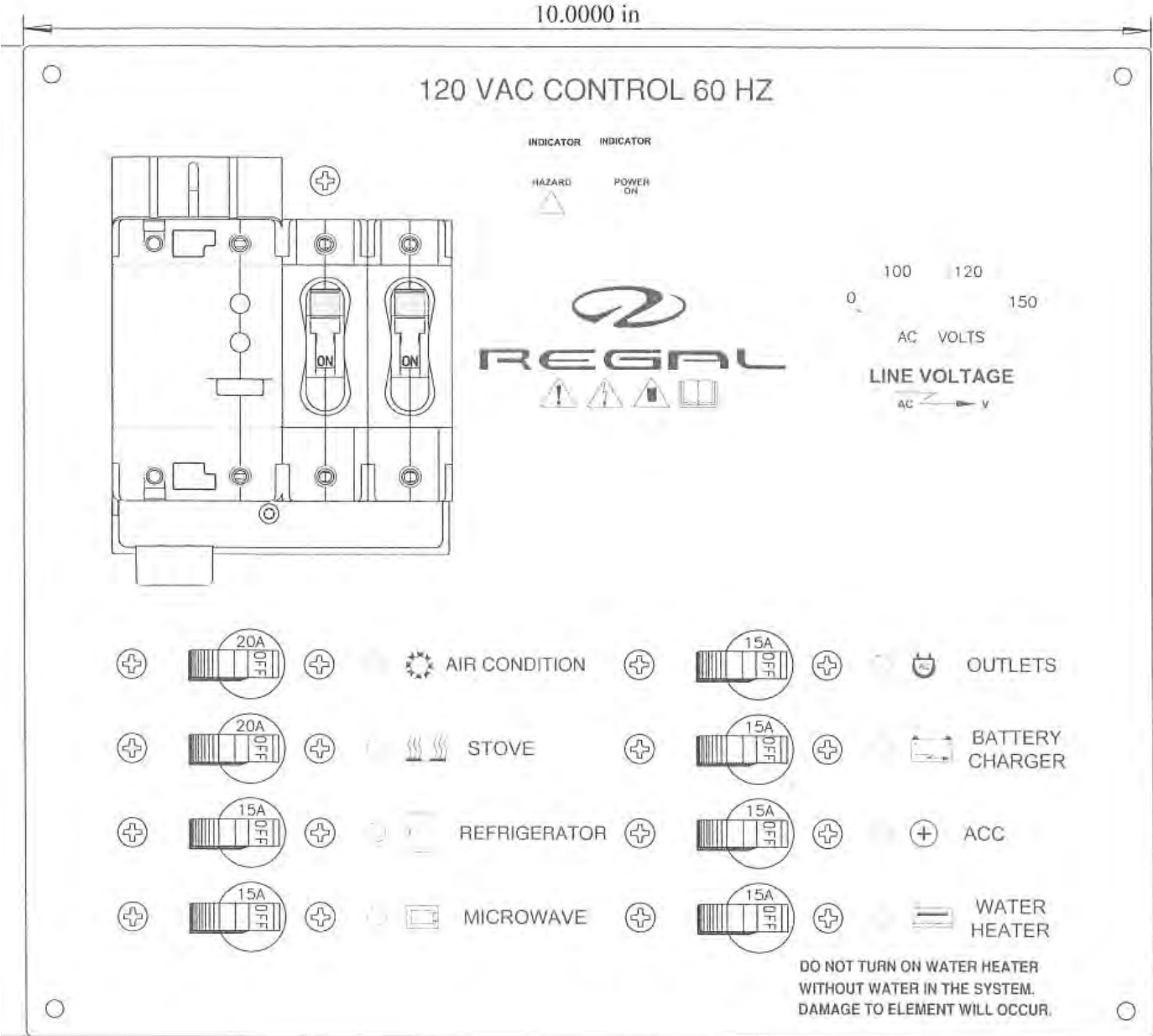
26 EXPRESS DOMESTIC 120 VOLT MAIN AC PANEL
