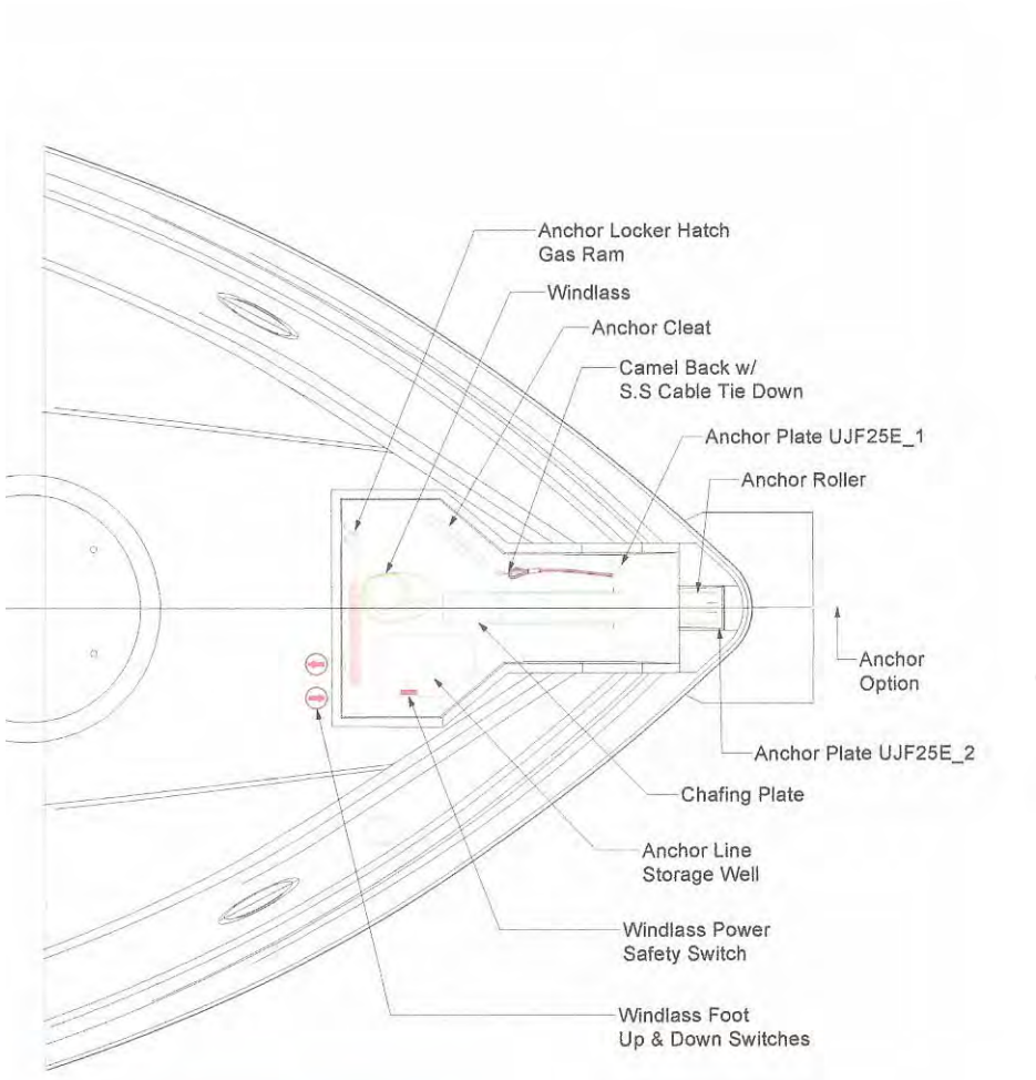
Deck Bow Plan
