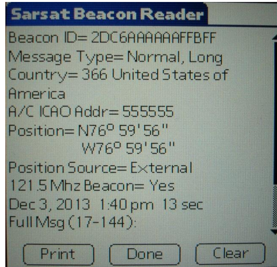
Figure 9: Example of 24-Bit Address Data View
