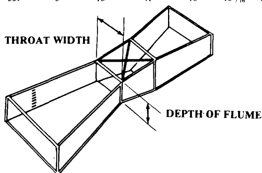
Figure 6.8 Parshall Flume
