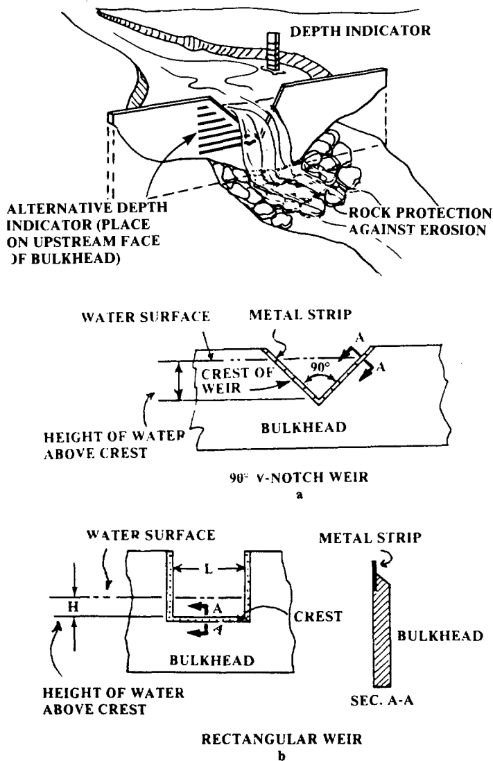
Figure 6.7 - Standard Weirs
