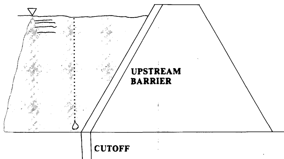
Figure 2.2 Embankment Dam
