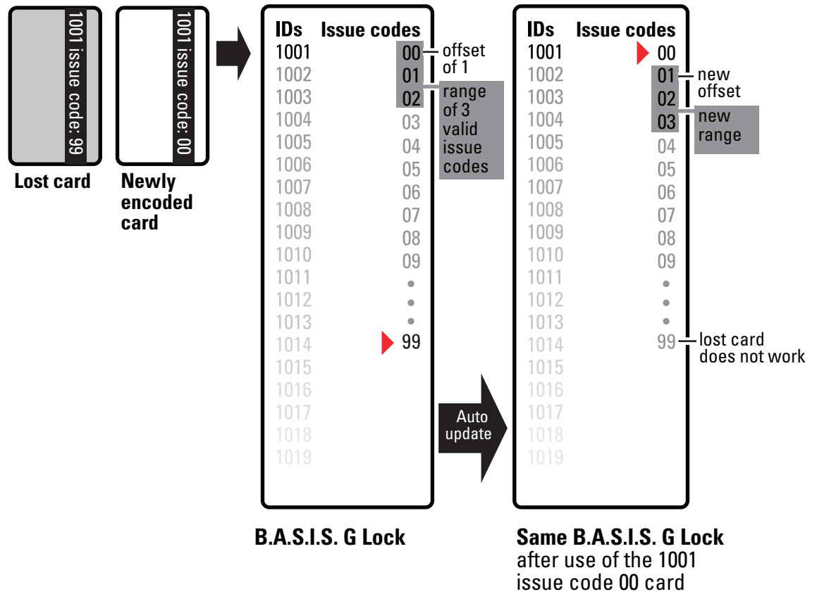
Figure 2.3 Guest functionality in rollover diagrammed
