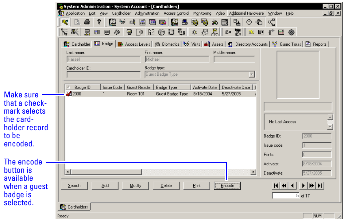
Figure 5.12 Getting ready to encode a guest badge
