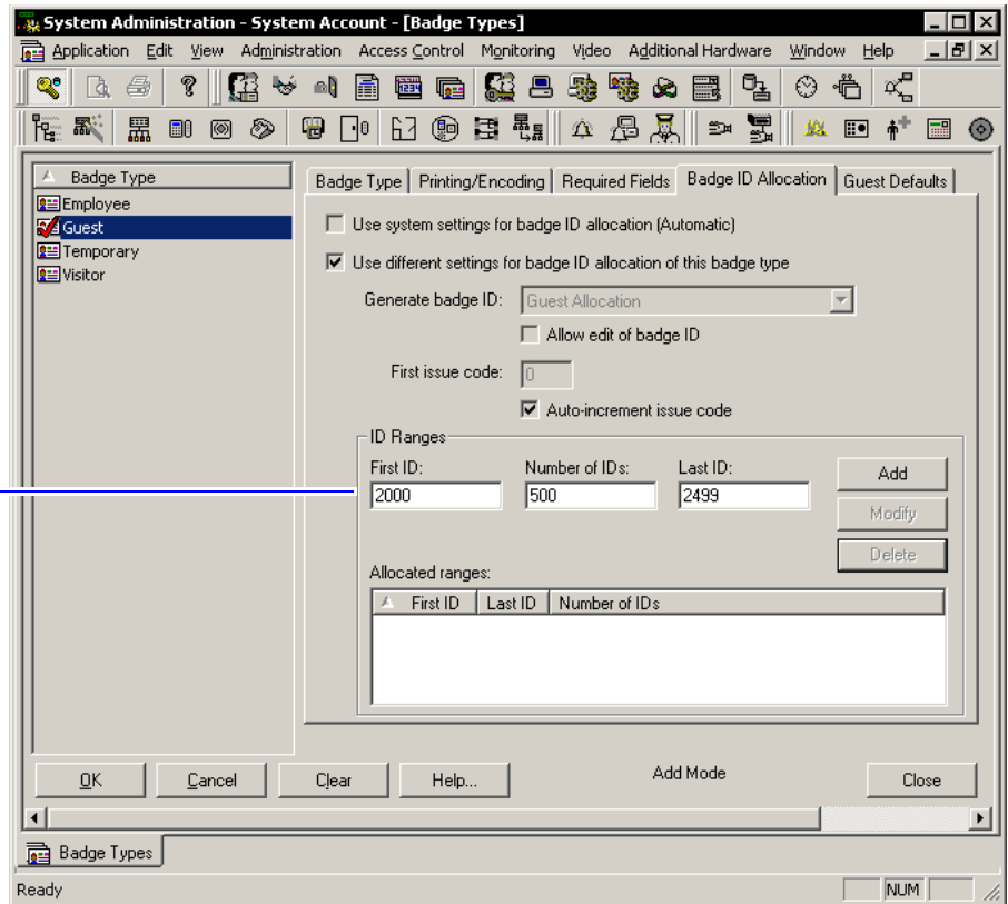
Figure 3.5 Entering the range of Badge IDs
