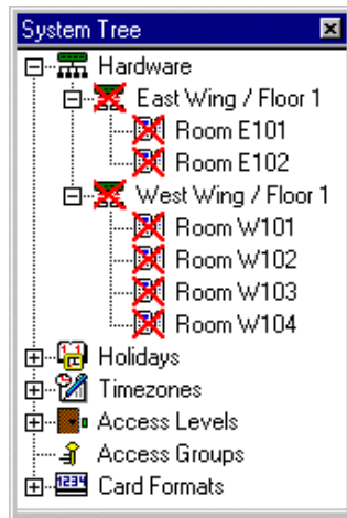
Figure 4.2 Expanding the System Tree to view readers
