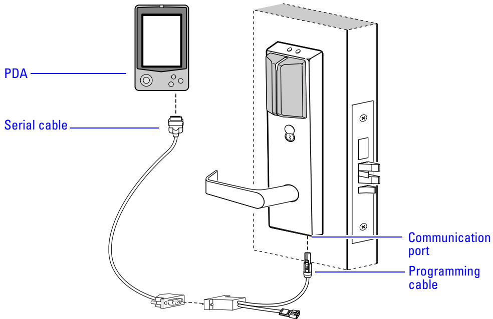
Figure 4.4 Connecting the PDA to a lock
