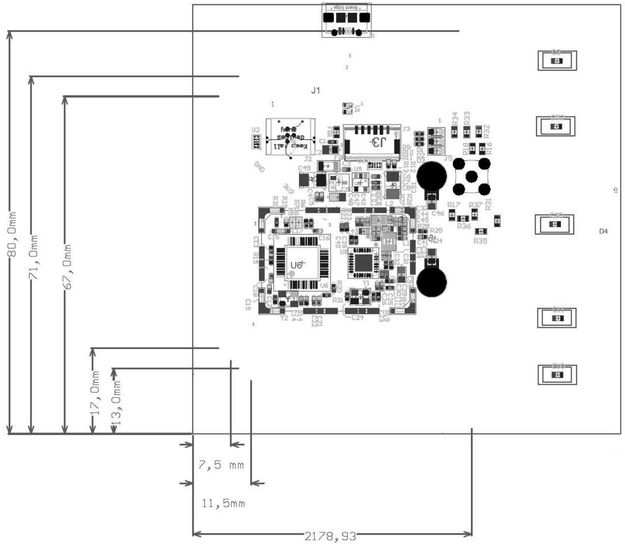
Figure 1: Top view of the eGym RFID Board v2
