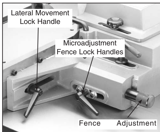
Figure 11. Fence controls.
