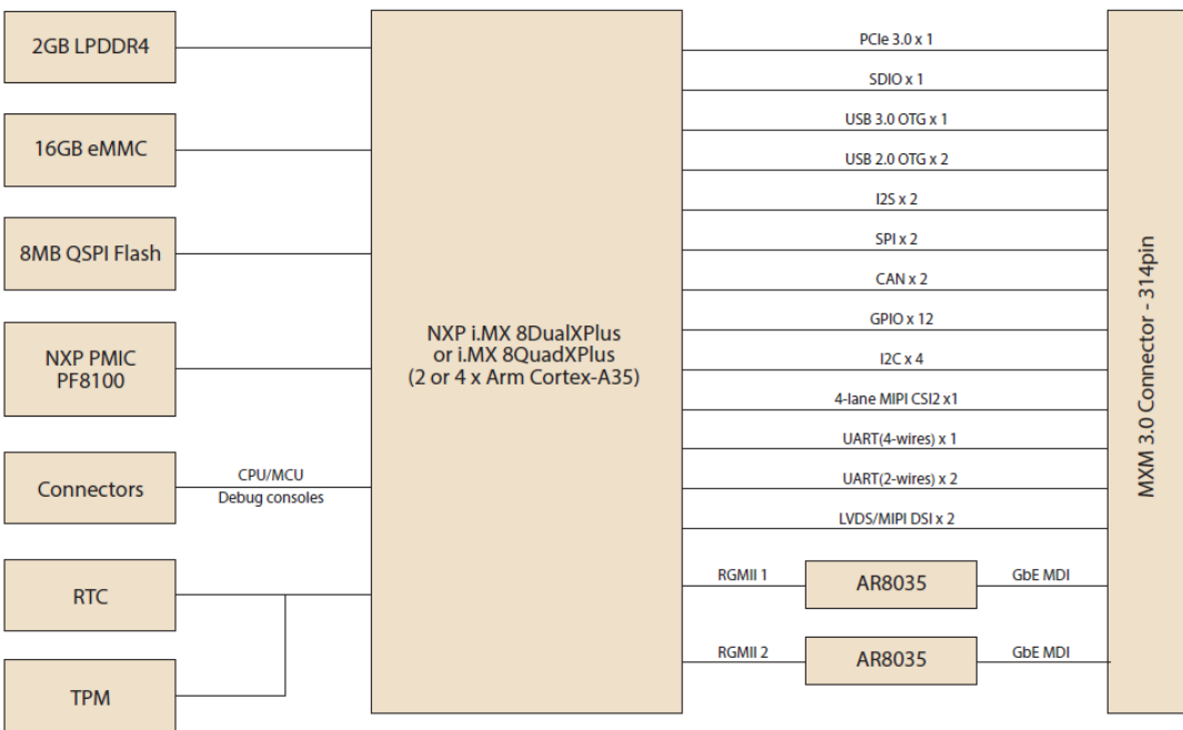
Figure 2.1 ROM-5620 Block Diagram
