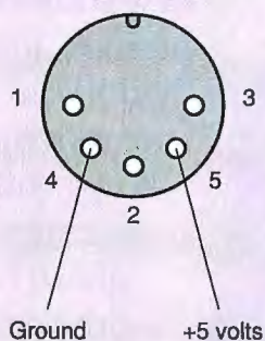
Figure A: To connect a Power Glove to your PC compatible, you need a 5-V power source. Pins 4 and 5 of a standard five-pin keyboard connector provide 5 V to the keyboard and can also be used to power the Power Glove.
