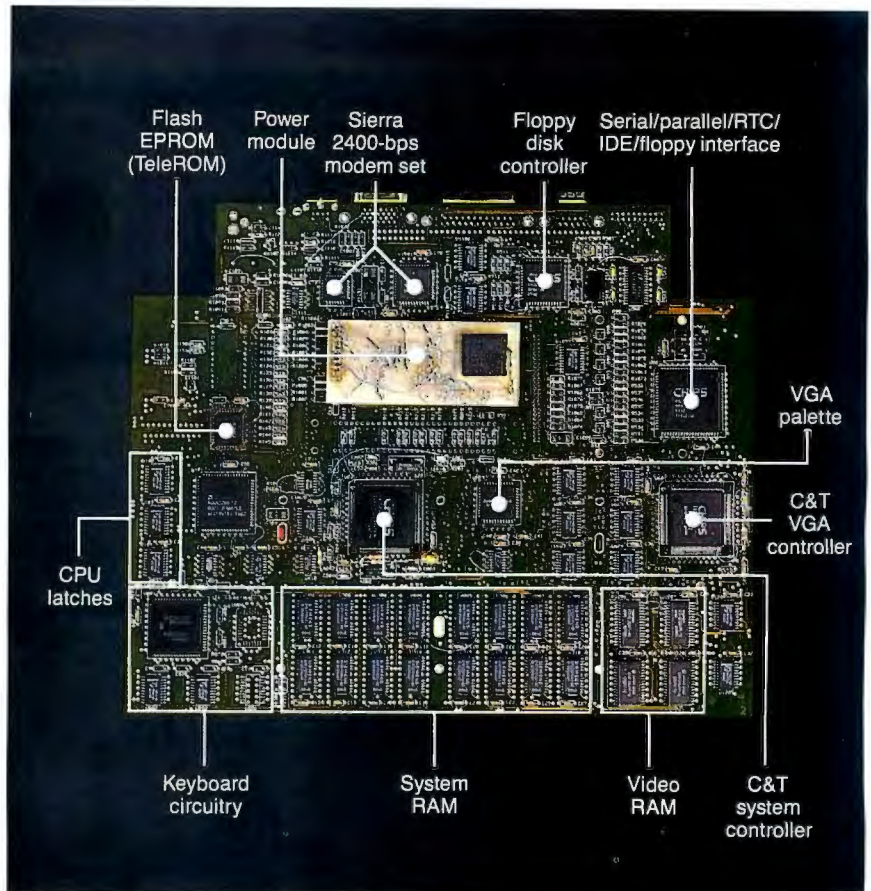
Photo 2: The VH-286 motherboard makes extensive use of surface-mount technology. It has a number of wire jumpers, which should not appear on the final production units.
