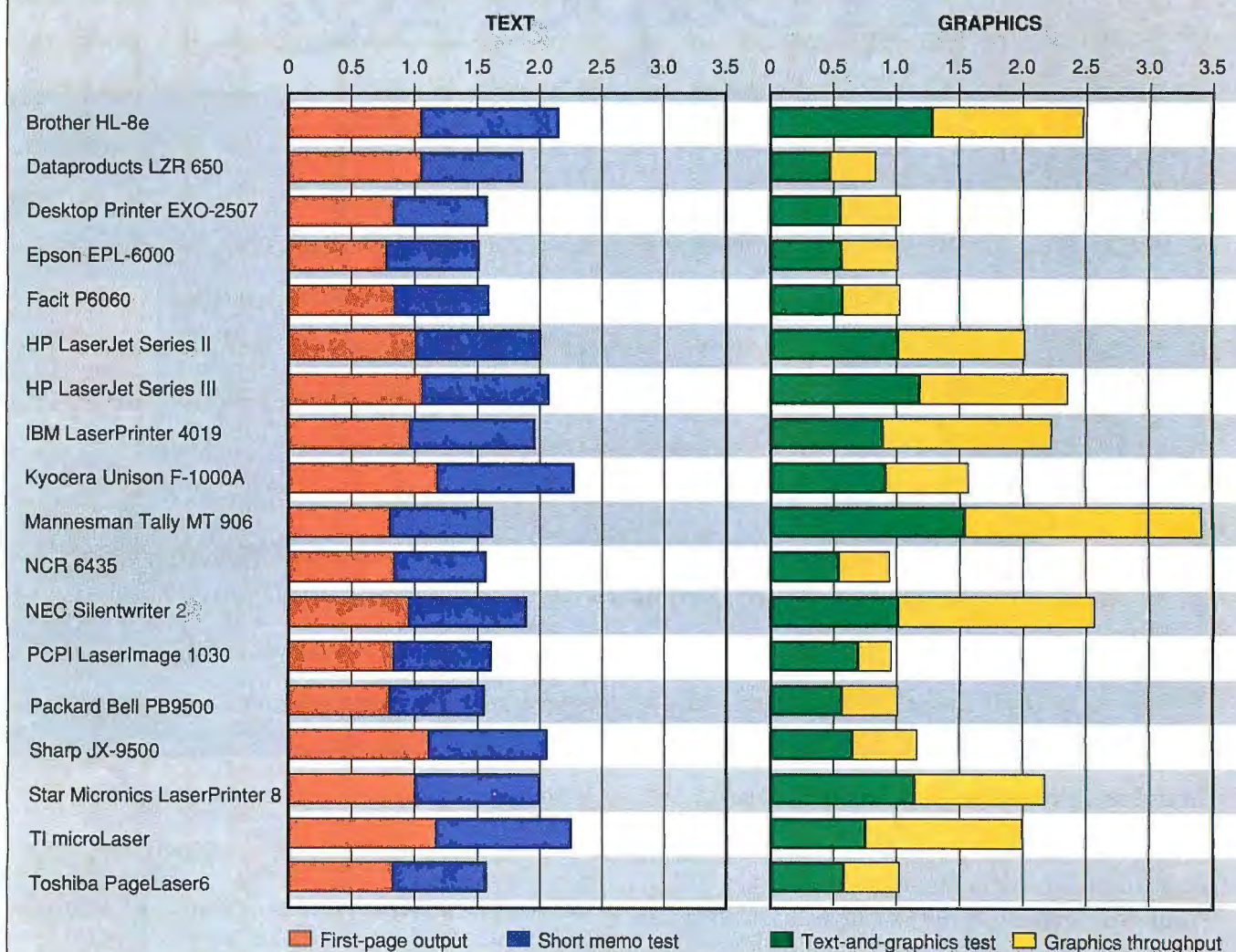
Figure 3: The Text Index combines two tests, the first-page output test and the short memo test. Use this index if your applications tend to be small, textual print jobs (e.g., memos, letters, and simple spreadsheets). The Graphics Index combines the text-and-graphics test and the graphics throughput test. Use this index if your applications include heavy-duty graphical elements—newsletters, flyers, complex spreadsheets, and scanned images. Use the Long Document Index if your print jobs tend to be many pages of pure text. In all cases, long bars indicate superior performance.
