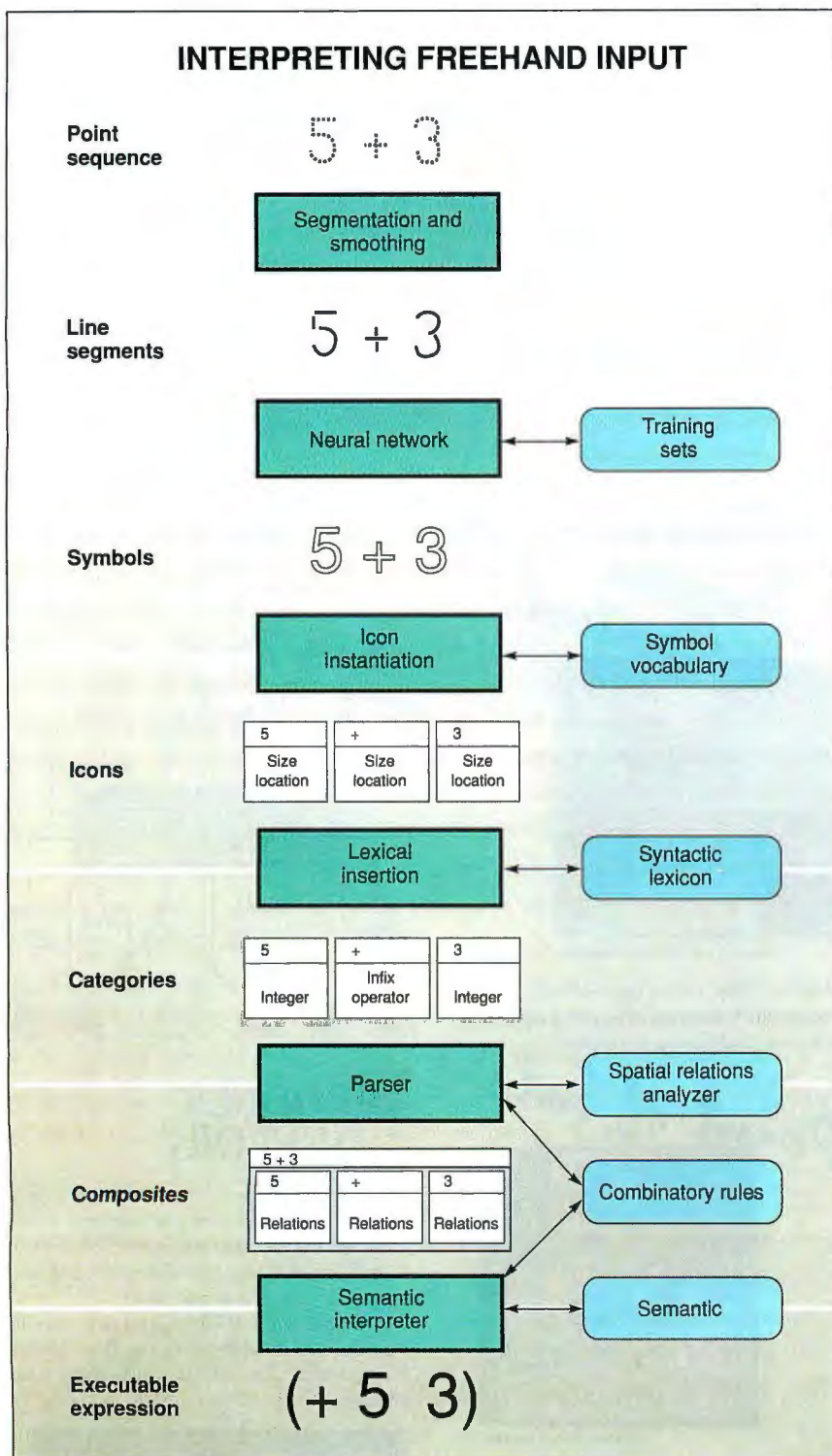
Figure 4: This figure shows how an interactive-tablet system interprets freehand input. The input is a digitized point sequence (shown at top); the result is an executable mathematical expression (shown at bottom). Knowledge sources in the middle column transform the data types in the left column using the data banks listed in the right column. Segmentation and recognition transforms the input into strokes and a set of symbols, respectively. Visual parsing works with symbol sets located in space (icons) and forms a composite expression using a visual grammar and lexicon. A semantic interpreter converts the parser output into an executable form.
