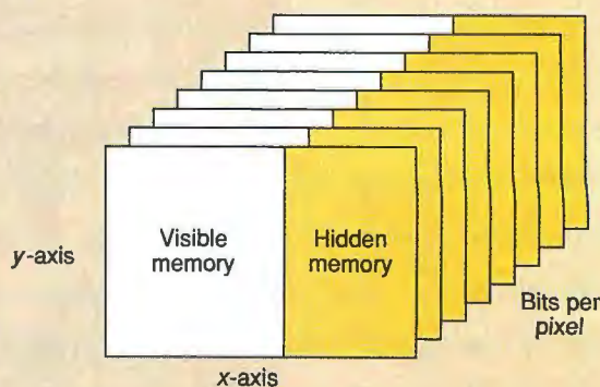
Figure 2: A graphical display with a single plane allows only monochrome images. Increasing the screen depth allows more colors, double-buffering for animation, z-buffering for 3-D rendering, alpha buffering for transparency, or antialiasing. The system shown here has 8 bits per pixel, which provides 2^8 options (256 color choices), and a portion of nondisplayable (hidden) screen memory, which can be used for fast generation of bit-mapped text, texture mapping, and pattern tiling.
