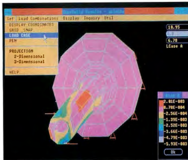
InerSolid, the stress-analysis module of Inertia, shows the results of analysis on a spindle.
