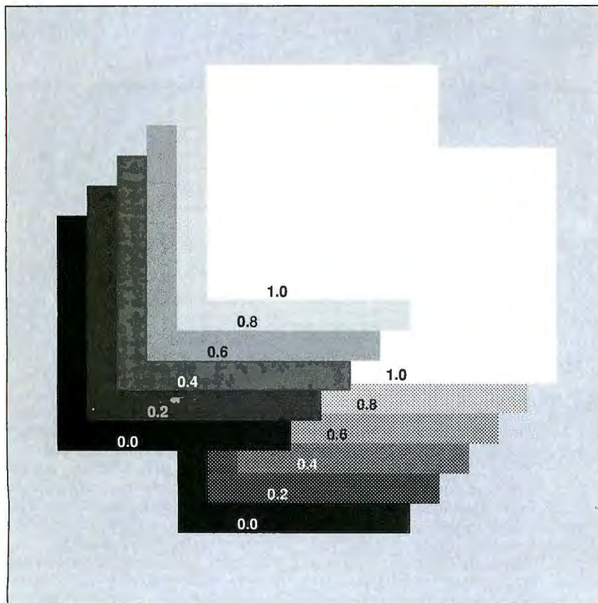
Figure 2: PostScript lets you vary grays by specifying the spot density and the angle of spot placement. Here, the lower set of grays is the printer default of 53 spots per inch and 45 degrees. The upper set is the optimum 106 spots and 45 degrees. The numbers in the squares represent the grayvalue.
