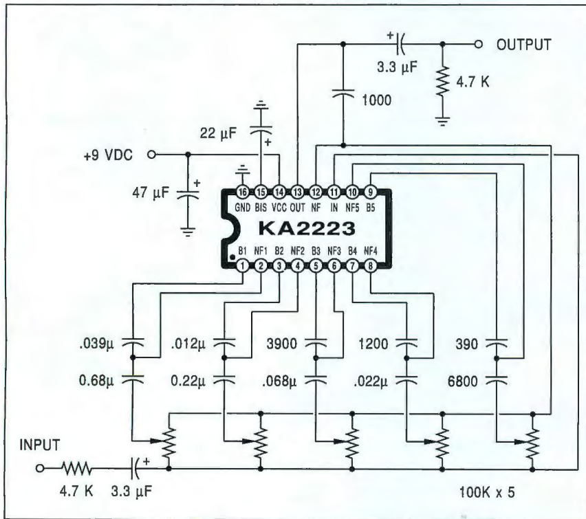
Figure 4: Opaque icons greatly simplify drawing PostScript electronic schematics, flowcharts, and other "blobs on strings" illustrations. All the background wires are continuous, and you slide them under the icons simply by placing them earlier in the text file. Line breaks are first printed as an opaque fat white line and then as a thin black line.
