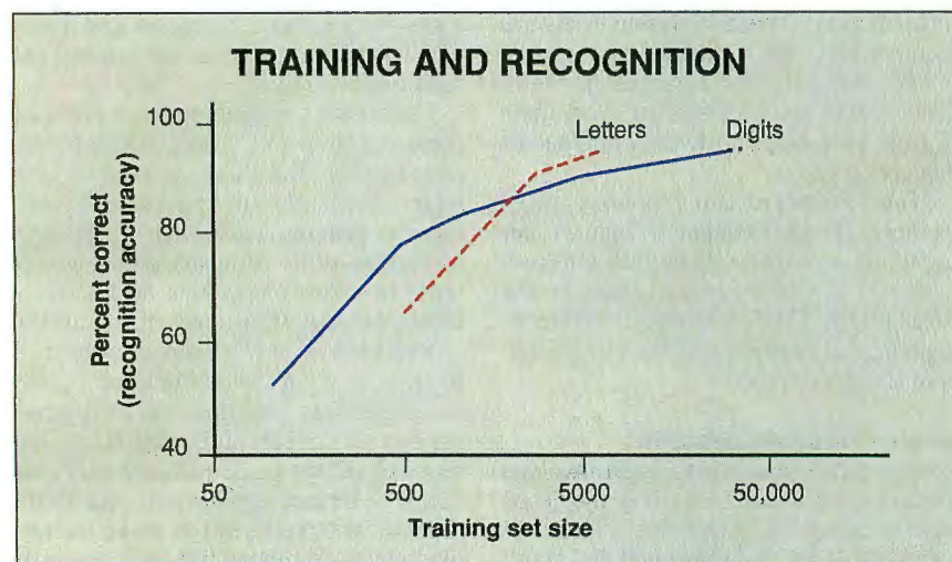
Figure 3: The figure plots accuracy rate versus the size of a training set for a back-propagation neural network. You need large training sets to achieve high accuracy rates.
