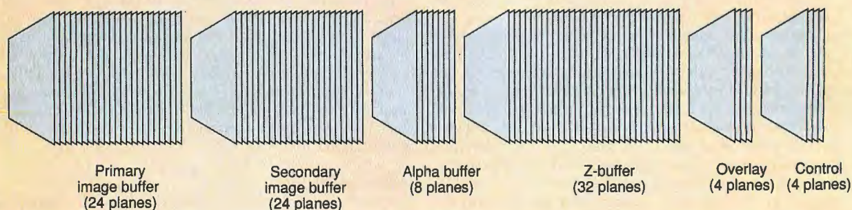
Figure 3: A frame buffer can have many bit planes and require a vast amount of memory. This configuration has a total of 96 bit planes. Assuming a screen resolution of 1280 by 1024 pixels, this represents 125,829,120 bits, or nearly 16 million bytes.
