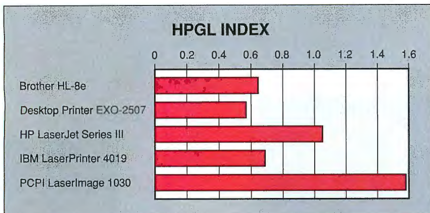
Figure 4: The HPGL Index. Three of the printers support the Hewlett-Packard Graphics Language internally. A fourth, the Desktop Printer EXO-2507, packages software emulation. The LaserJet Series III, driven by HP's latest incarnation of its Printer Control Language (PCL 5), incorporates HPGL commands into its command set. The index is based on the Series III results. Long bars indicate superior performance. The PCPI LaserImage 1030 produced the sharpest plots in record time.
