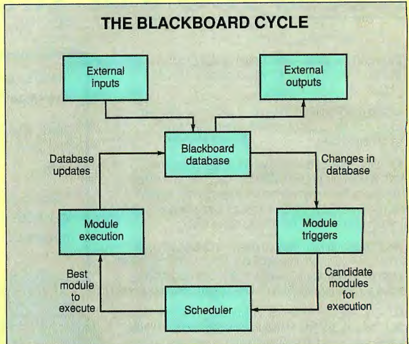
Figure A: A blackboard system lets multiple modules work on the same input. In an interactive-tablet system, the modules might consist of a neural network, lexical insertion, and a spacial parser.
