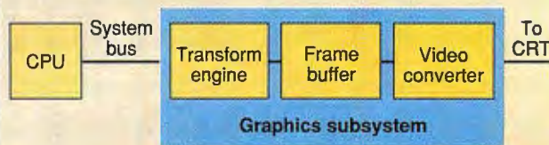
Figure 1: When dealing with a 3-D model, the system's main CPU passes the information about the object to the transform engine (in the graphics subsystem). This specialized floating-point processor converts the information into the 2-D screen image, which is stored in the frame buffer. The video converter reads the frame buffer to create video scan information.
