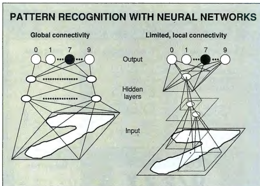
Figure 1: Back-propagation techniques enable a neural network that starts out with randomly valued connections to learn to correctly recognize input patterns. Network architectures with limited connectivity represent one way to make these recognition systems compact enough to fit on small machines.
