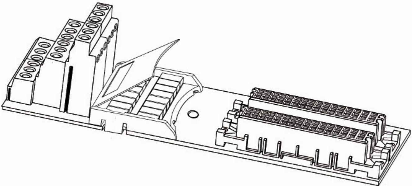
Figure 5 - Single Termination Assembly
