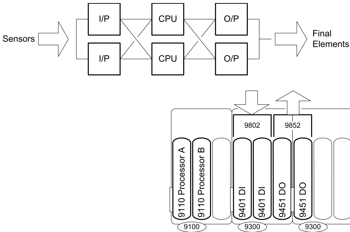
Figure 15 - Dual Inputs, Processor and Output System
