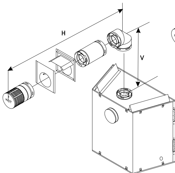
Figure 10. Venting with One 90° Elbow
