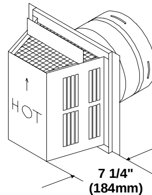
Figure 26. Round & Trapezoid Termination Caps
