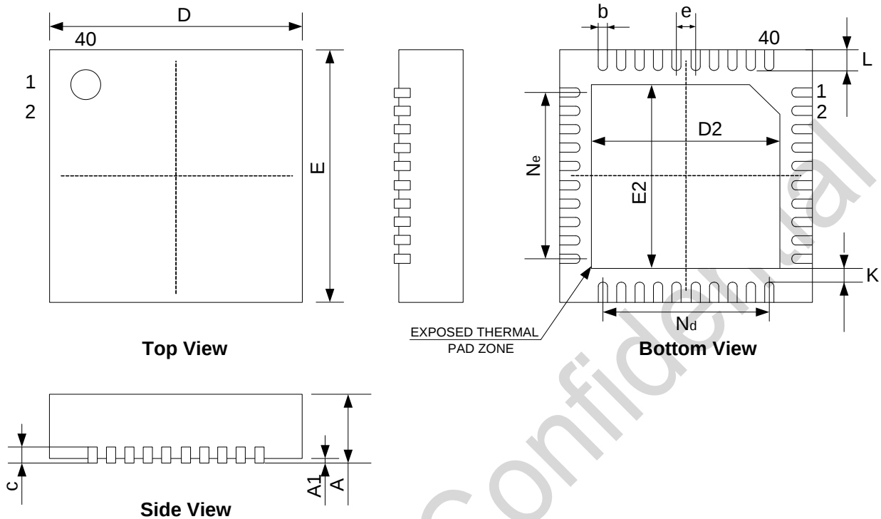
Figure 33. QFN405x5 Packaging
