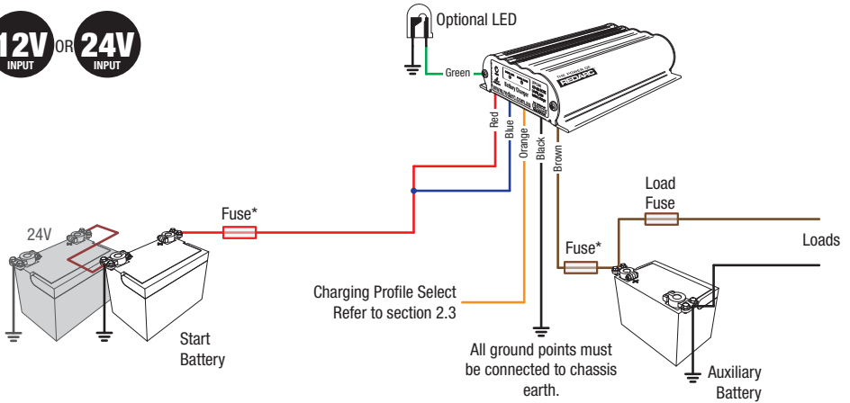
Figure 2.8a - BCDC1225 and BCDC1240 Standard setup for a 12V or 24V Start Battery
