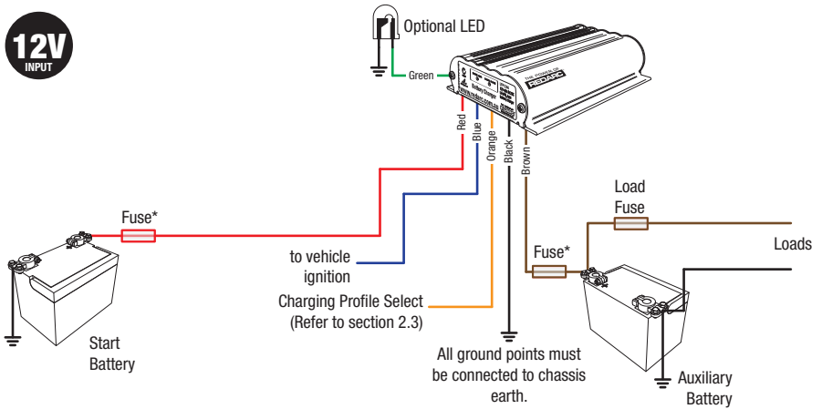
Figure 2.8b - BCDC1225-LV and BCDC1240-LV Standard setup for a 12V Start Battery
