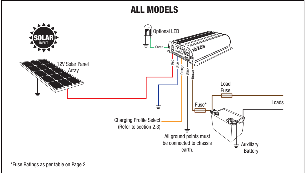
Figure 2.8c - All Models Standard setup for a 12V Solar array
