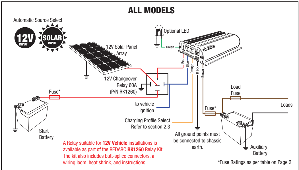
Figure 2.8d - Using a changeover relay for 12V Start Battery & 12V Solar array inputs
