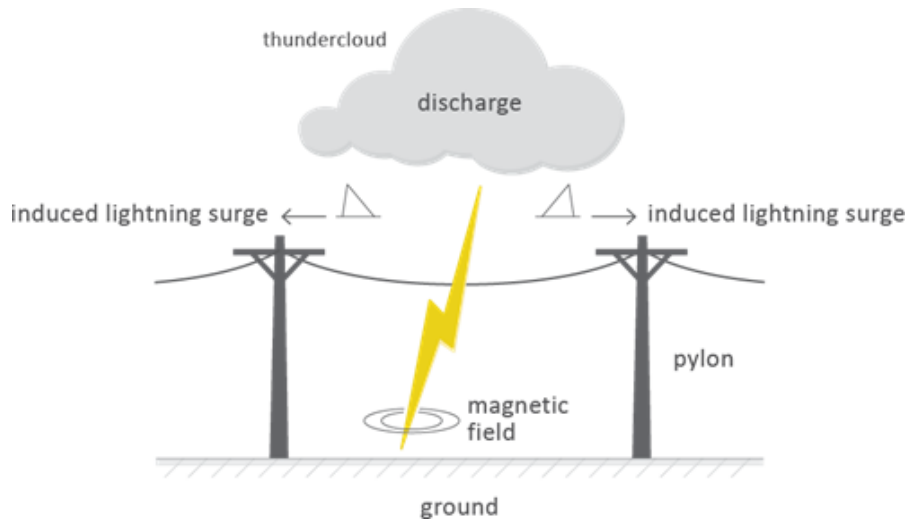
Figure 5: Electromagnetic induction
