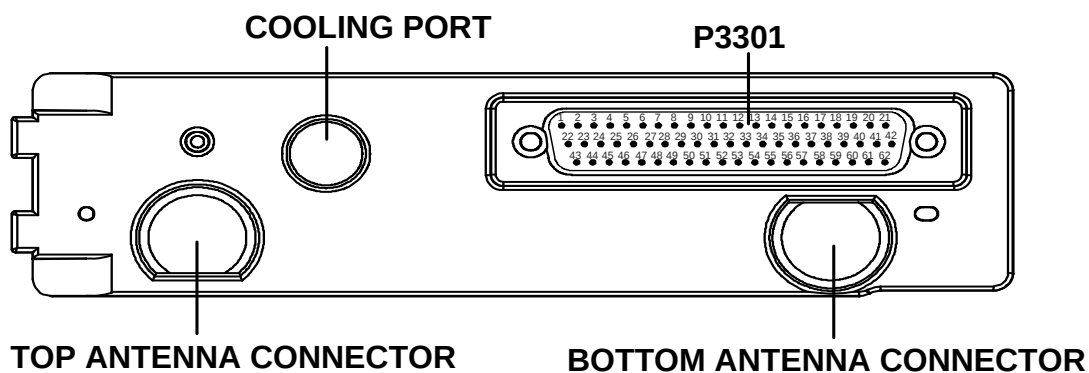
Figure 5-29. GTX 33 Backshell Connectors
