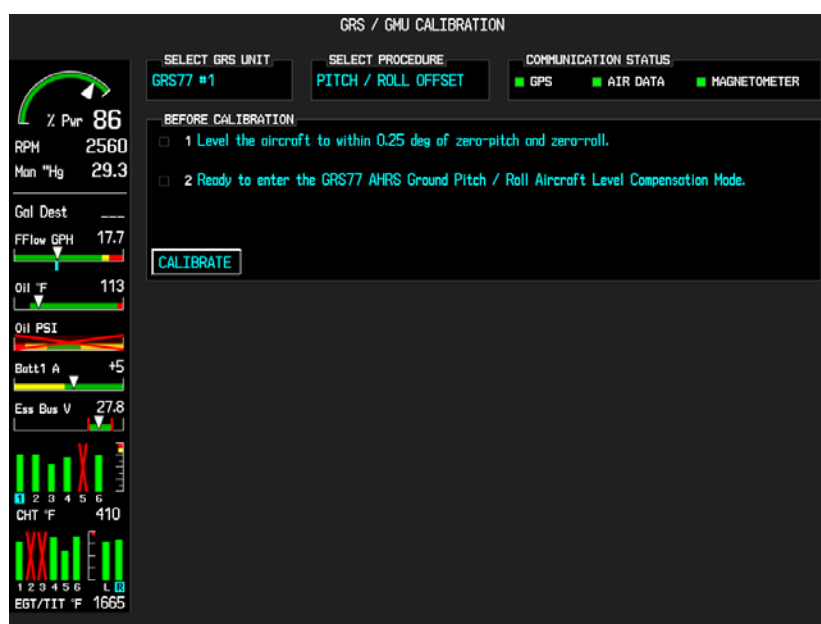
Figure 7-7. GRS/GMU Calibration Page
