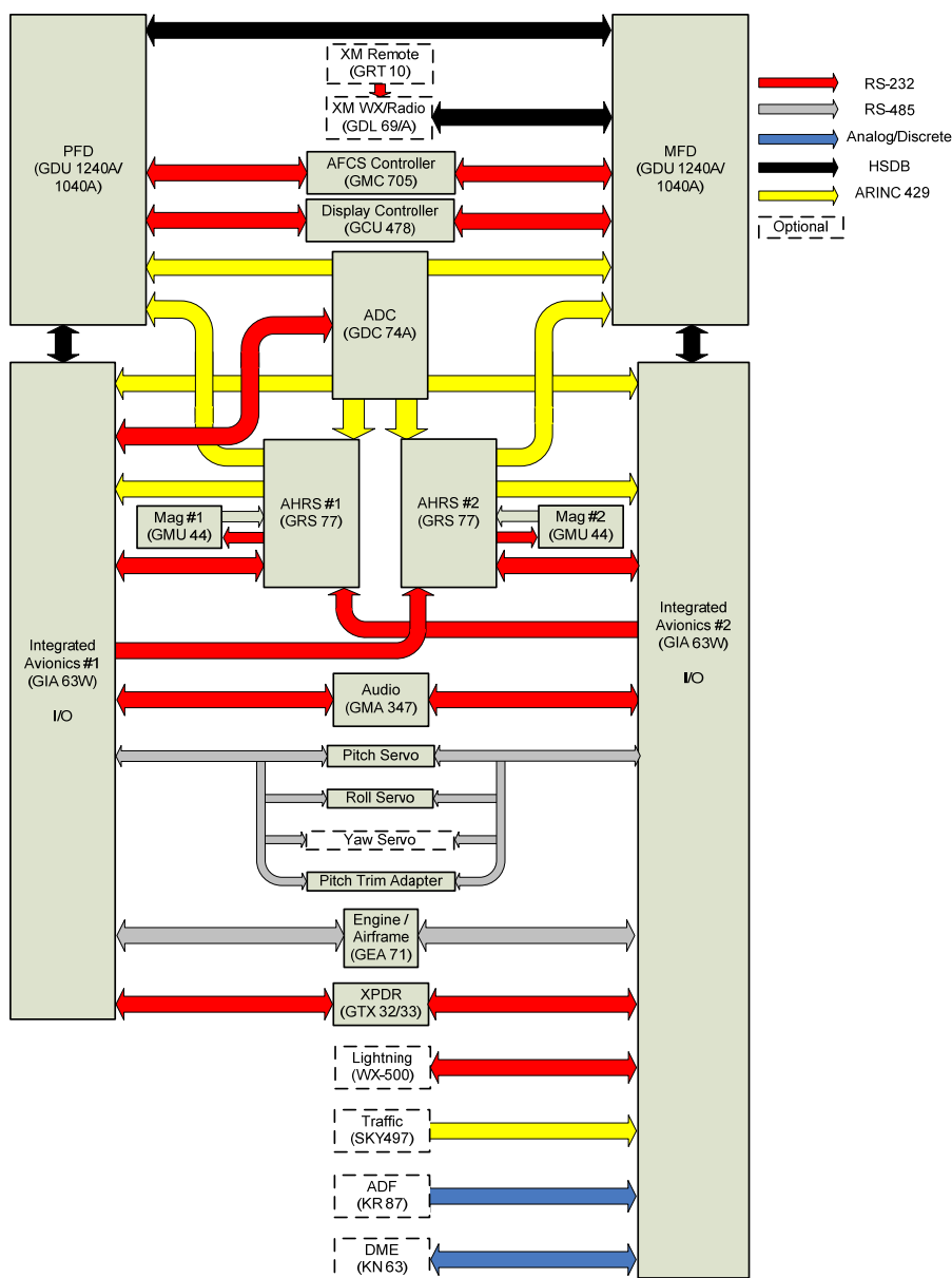
Figure 3-1. Dual AHRS, Single ADC Configuration
