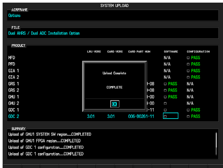
Figure 10-4. Dual AHRS Option
