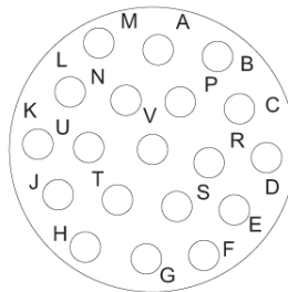
Figure 5-36. GSA 80/81 Backshell Connector (P801)
