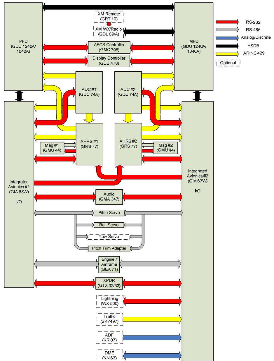
Figure 3-2. Dual AHRS, Dual ADC Configuration
