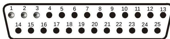
Figure 5-38. GTX 32 Backshell Connector (P3271)
