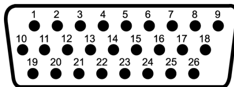
Figure 5-37. GTA 82 Backshell Connector (P821)
