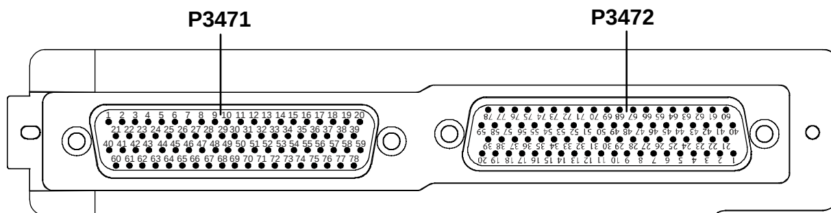
Figure 5-28. GMA 347 Backshell Connectors
