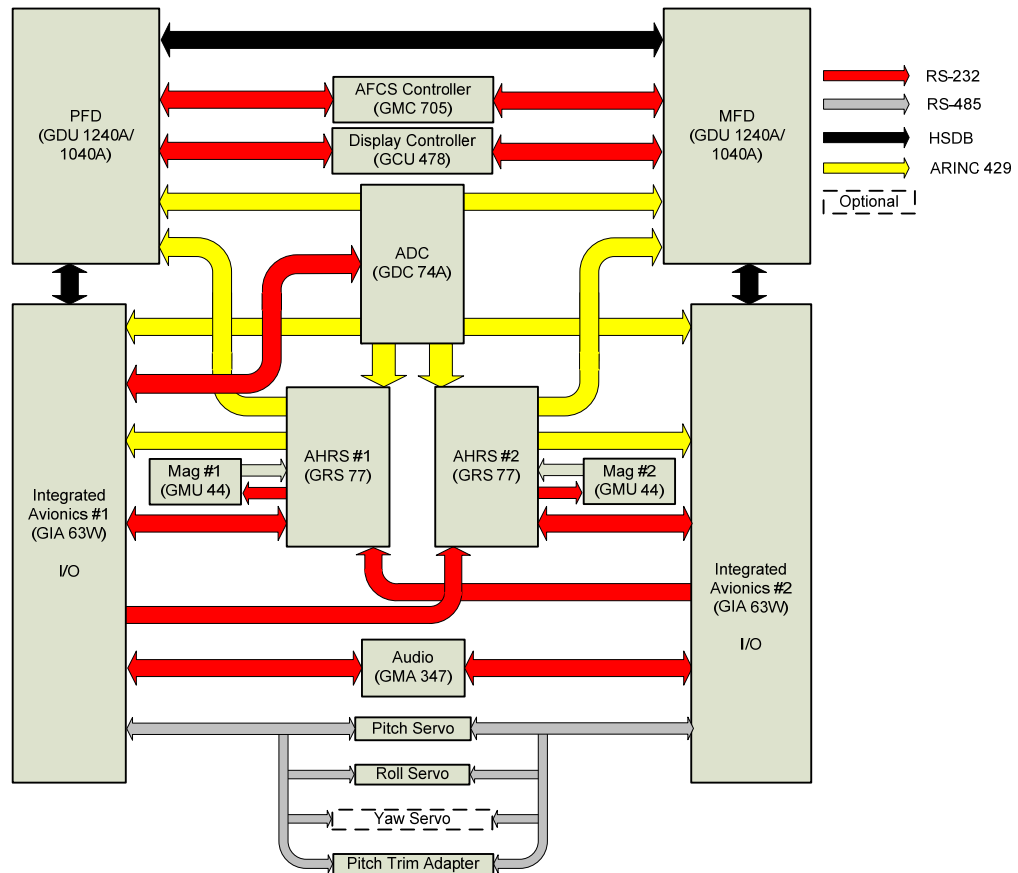
Figure 3-3. GFC 700 System Interface
