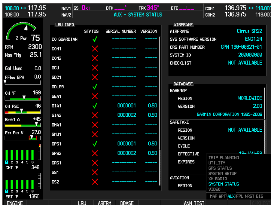
Figure 5-3. System Status Page (AUX Group)
