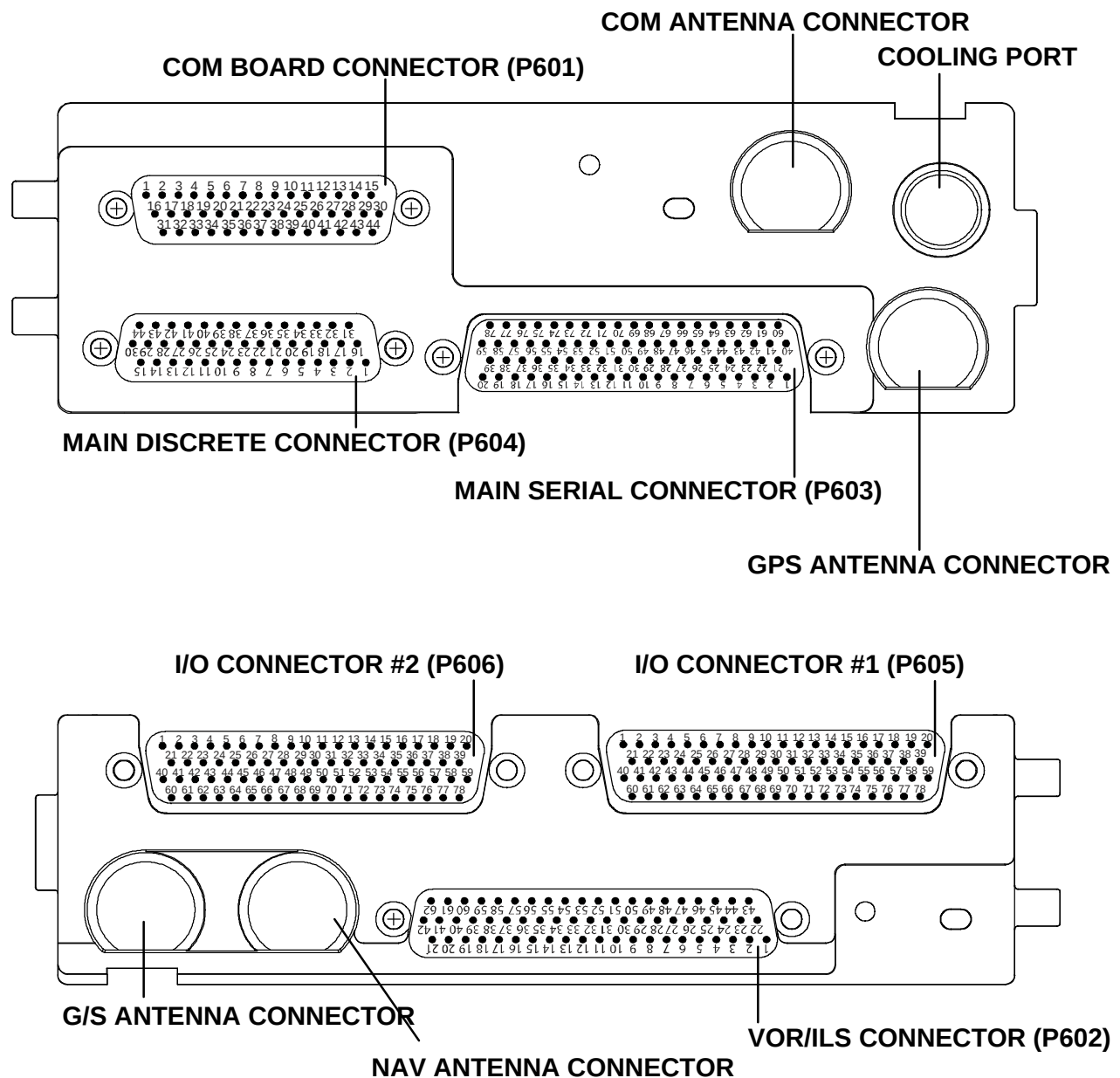
Figure 5-26. GIA 63W Backshell Connectors
