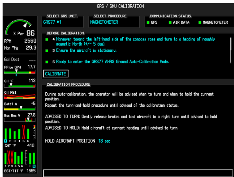
Figure 7-9. GRS/GMU Calibration Page
