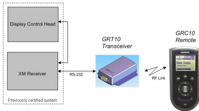
Figure 2-17. GRT 10 Remote Controller and GRC 10 Wireless Transceiver
