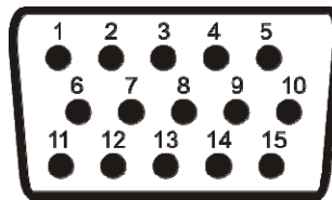
Figure 5-34. GMC 705 Backshell Connector (P7101)
