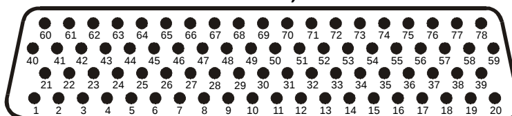
Rear Connectors J3471 and J3472, Viewed From Back of Unit
