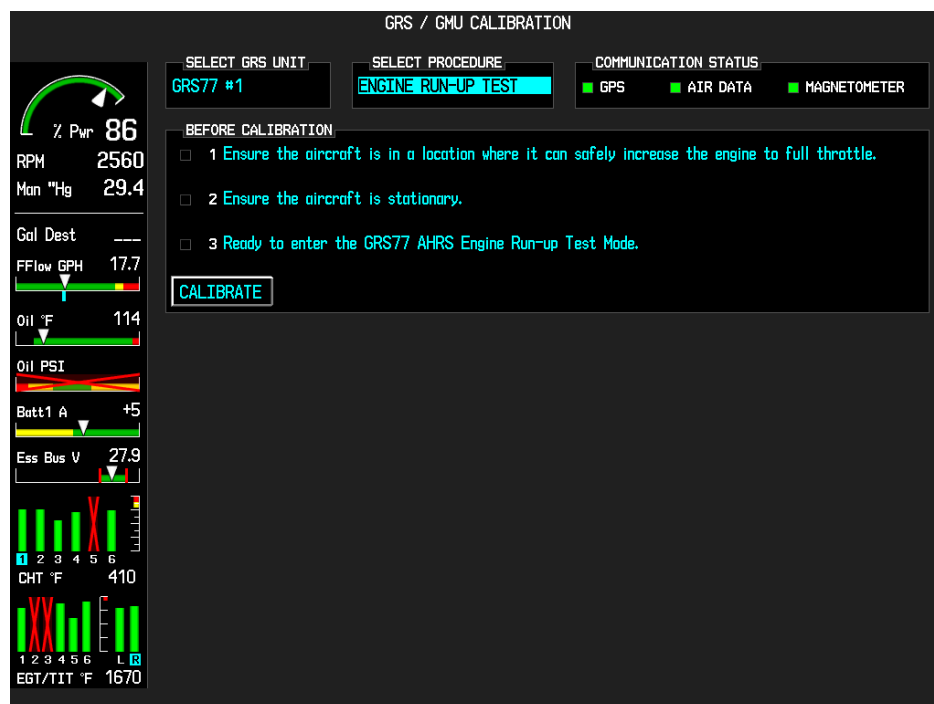
Figure 7-10. Engine Run-Up Test Display
