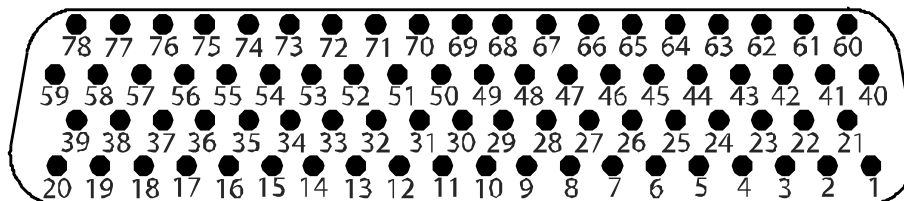
Figure 5-32. GDC 74A Backshell Connector (P741)
