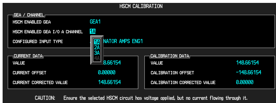
Figure 5-21. HSCM Enabled GEA I/O A Channel Selection Box
