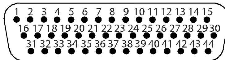
Figure 5-31. GRS 77 Backshell Connector (P771)
