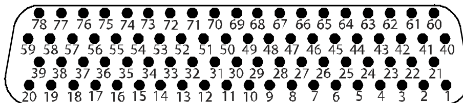
Figure 5-33. GDL 69A Backshell Connector (P691)
