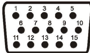
Figure 5-35. GCU 478 Backshell Connector (P4751)
