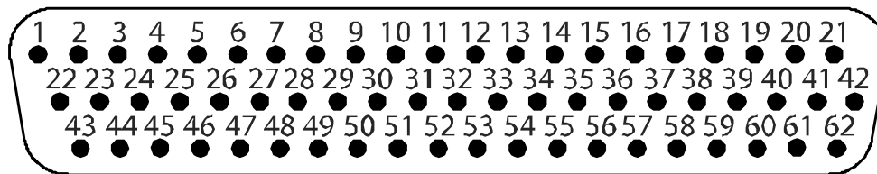
Figure 5-30. GDU 1240A Backshell Connector (P10001)
