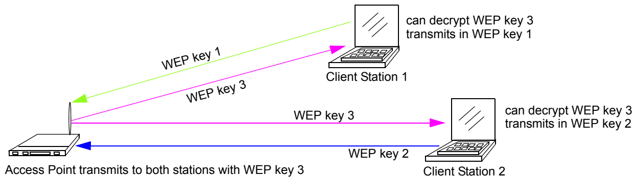
Figure 9. Example of Using Multiple WEP Keys and Transfer Key Index on Client Devices
