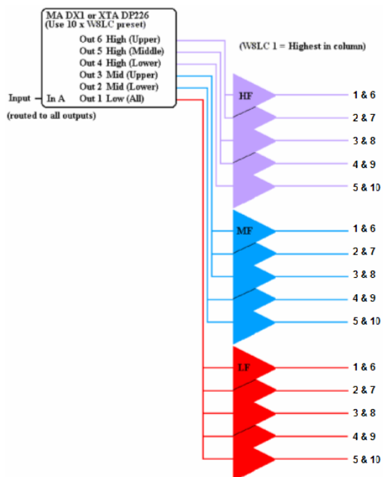
Standard W8LC amplifier rack for 10 x W8LC using standard 10W8LC High Curve preset (Individual lf, mf & hf shown)
