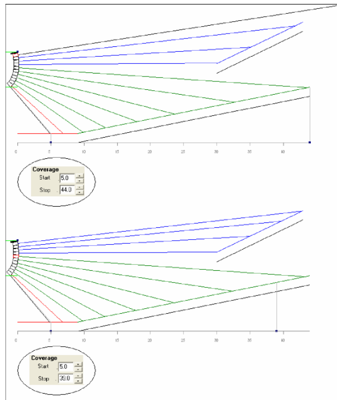
Reducing echoes by trimming the coverage stop
