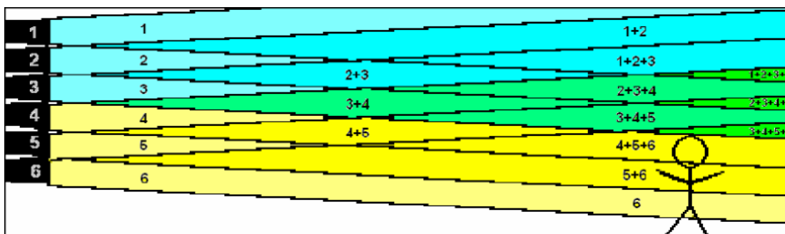
6-cabinet line array showing very simplified 7.5deg mid-HF coverage
