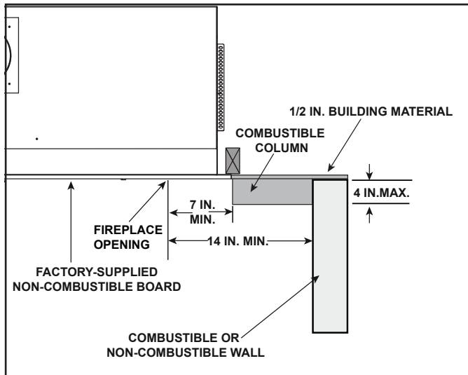
Figure 10.7 Combustible Mantel Leg and Wall Projections
