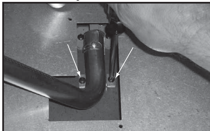
Figure 11.18 Remove Outside Burner Tubes
