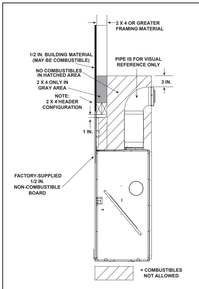
Figure 10.11 Non-Combustible Zone
