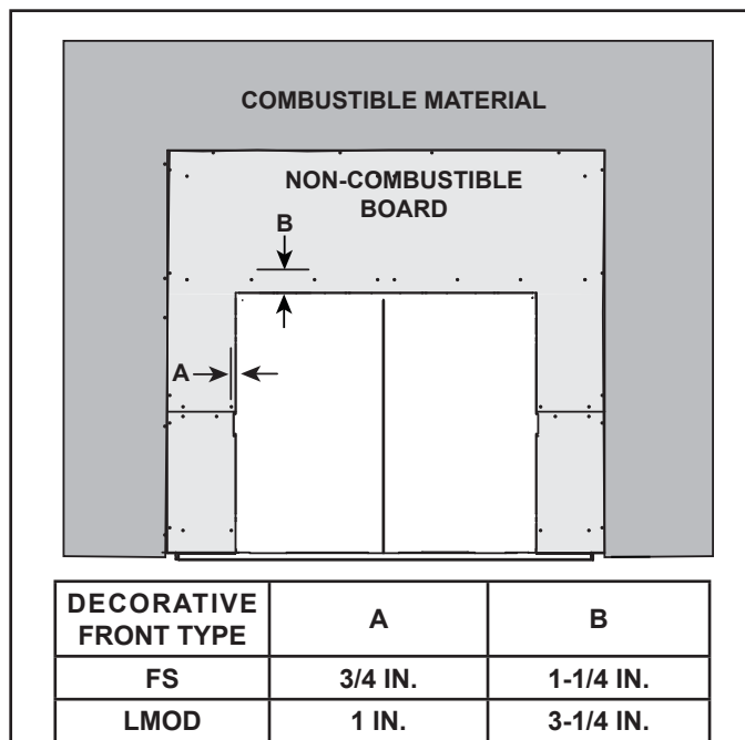
Figure 10.12 Required Clearance for Inside Fit Decorative Fronts
