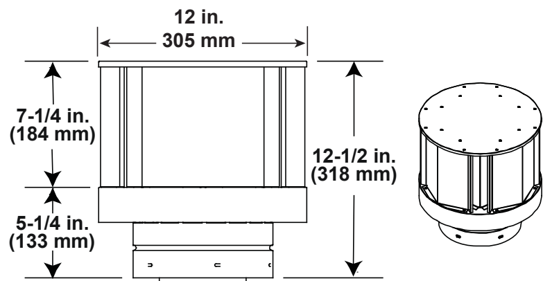
DVP-TVHW Vertical Termination Cap (Highwind)
