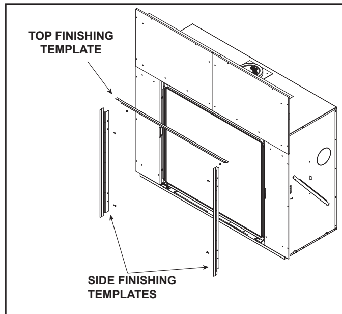
Figure 10.2 Top and Side Finishing Template Locations
