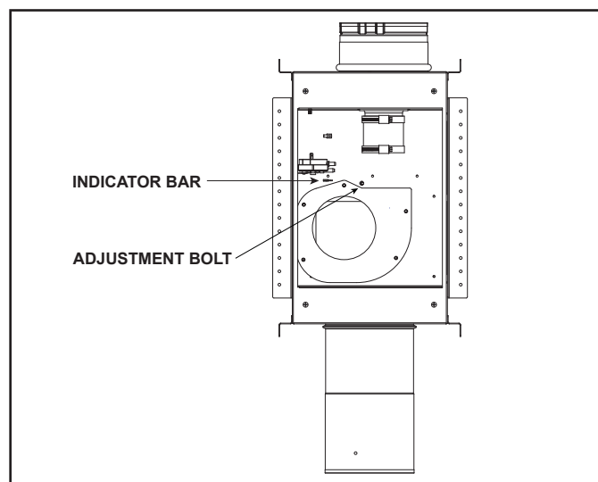
Figure 4.12 Baffle Adjustment Location - PVI-SLP
