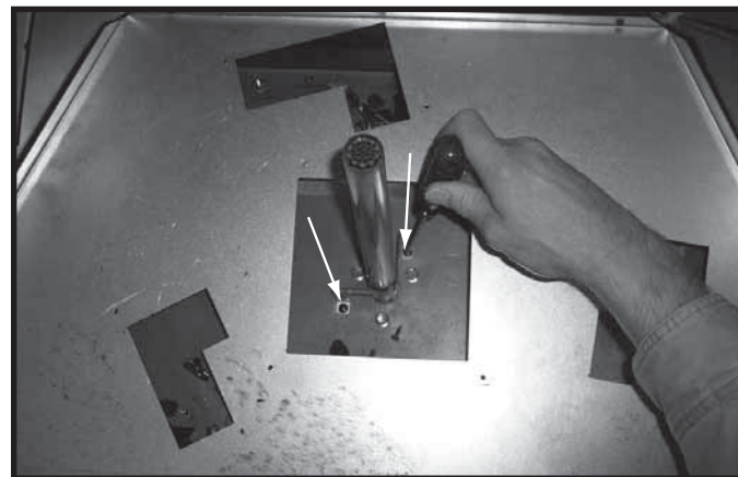
Figure 11.20 Remove Center Burner Tube
