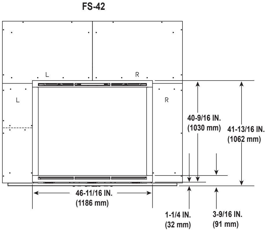
Figure 3.4 Decorative Front Dimensions (LUX42)
