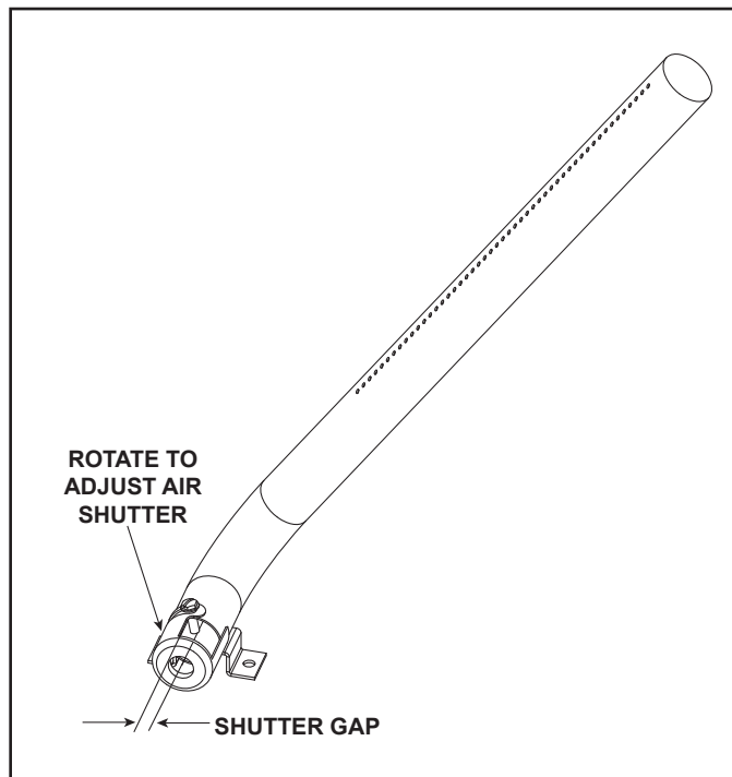
Figure 9.1 Air Shutter
