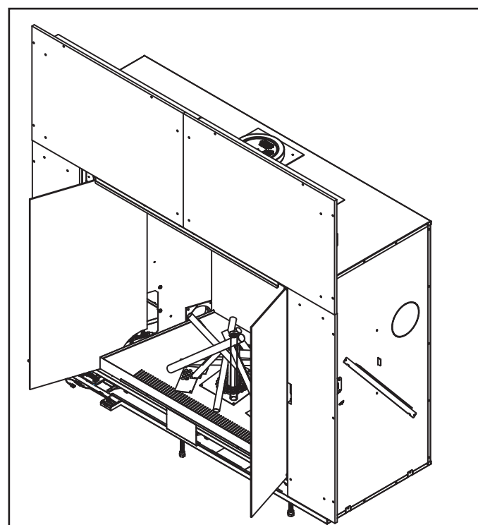
Figure 11.11 Side Panel Installation
