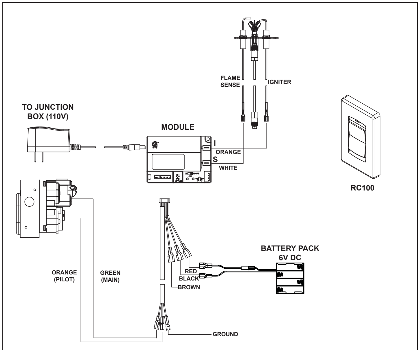
Figure 8.3 IntelliFire Pilot Ignition (IPI) Wiring Diagram
