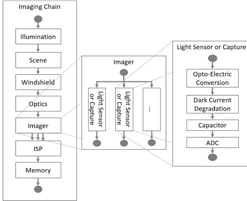
Figure 11 Example flow diagram of an imaging chain 6
