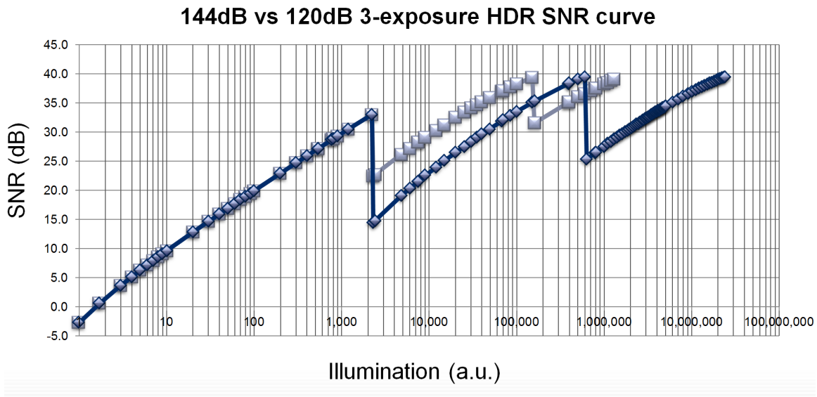
Figure 8 SNR vs. illumination for multi exposure HDR imagers
