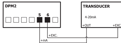
2 WIRE CONNECTION WITH EXCITATION SUPPLIED BY THE DPM2
