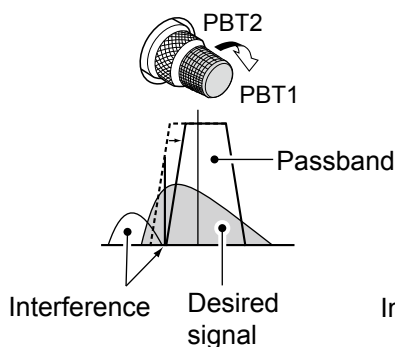
Cutting the lower passband
