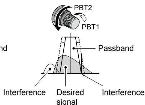
Cutting both higher and lower passbands
