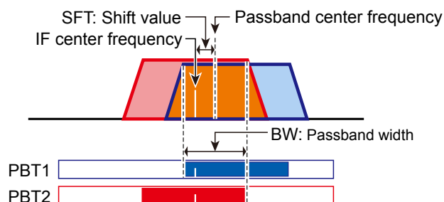
Cutting both higher and lower passbands
