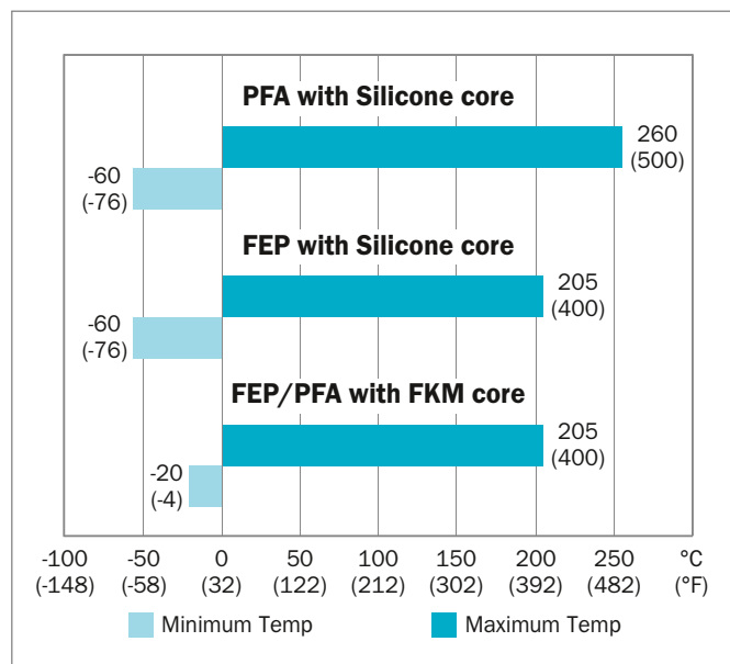
Figure 37: Temperature range
