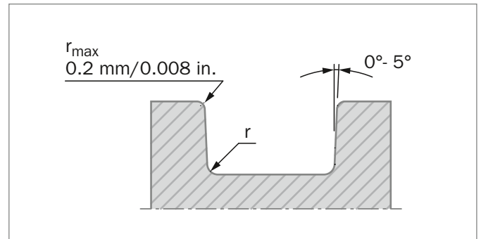
Figure 26: Groove specifications
