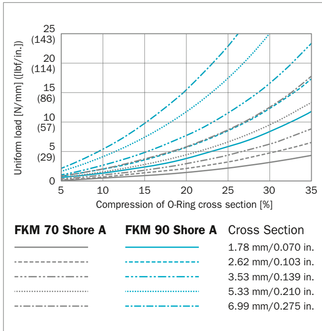
Figure 20: Guiding values for the uniform load [N/mm] ([lbf/in.]) of compressed O-Rings, material types FKM 70 Sh A and FKM 90 Sh A
