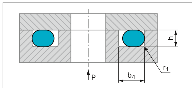
Figure 50: Axial installation, static, inside pressure
