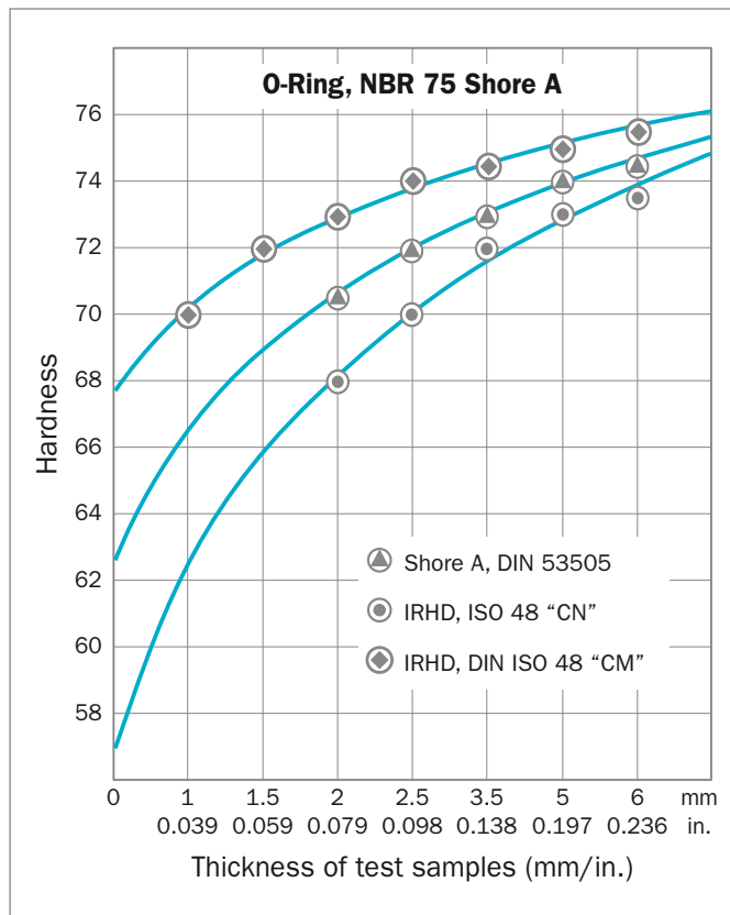
Figure 7: Ranges of hardness depending on sample thickness and test method
