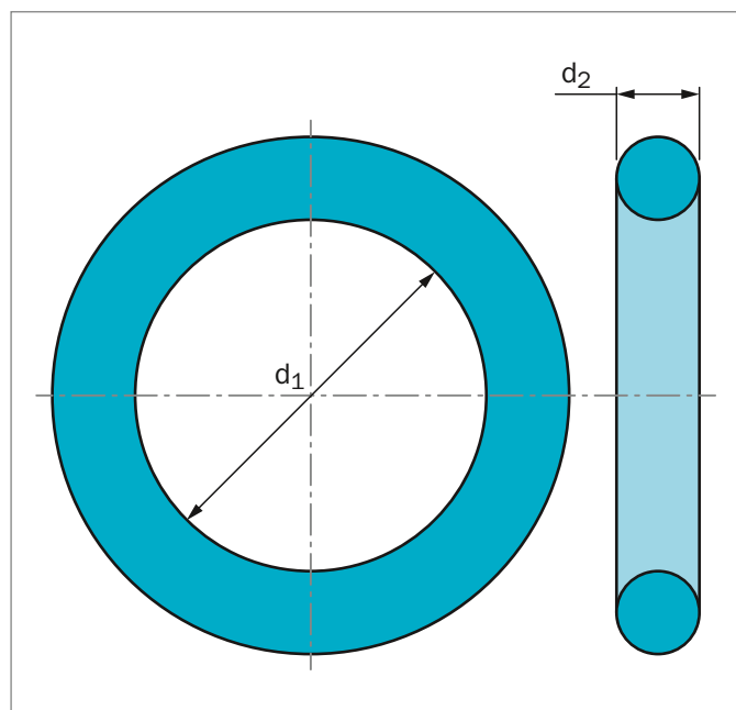
Figure 1: O-Ring dimensioning
