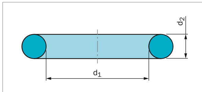
Figure 33: O-Ring dimensions
