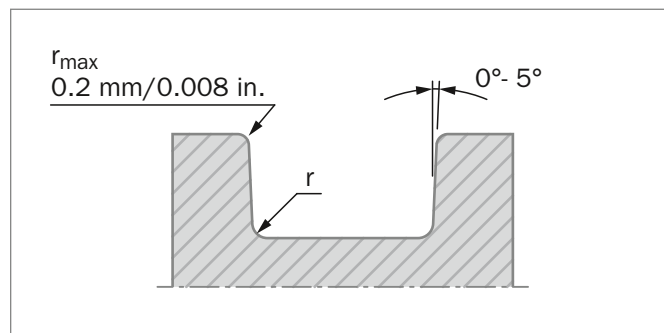
Figure 41: Rectangular housing groove design cross section
