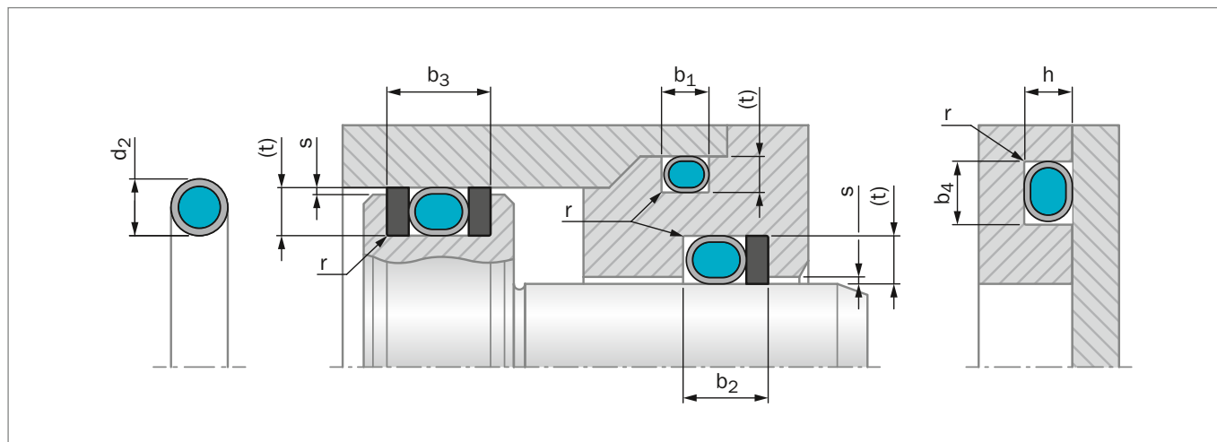
Figure 44: Installation drawing
