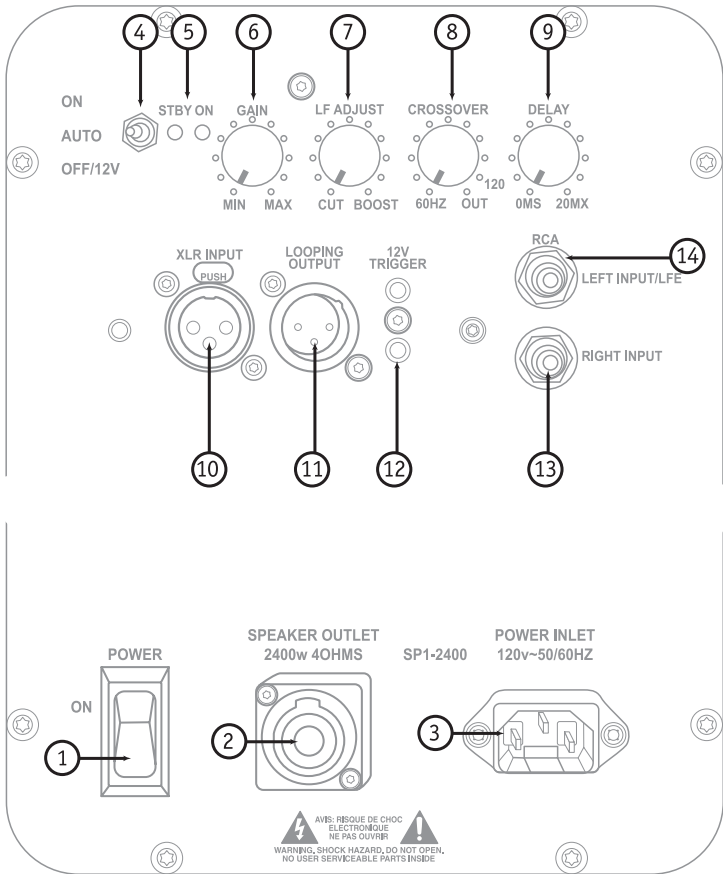
Signature SV Series Subwoofer Diagram for the SV-1212PR (2400 Watt Amplifier).
