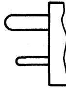
Figure D-5. Plug with Earthing (Ground) Pin – 13-A Max, 250V (U.K.)
