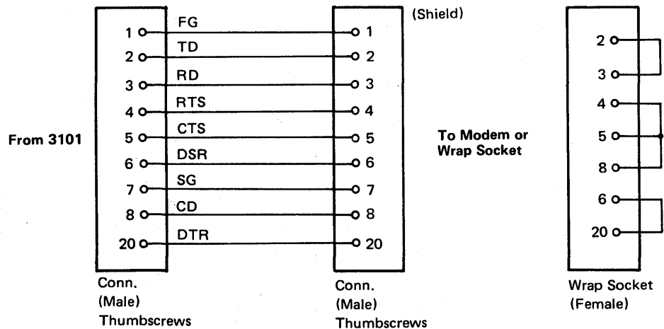
CCITT Modem Cable - 3.0 m
