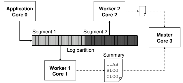
Figure 3: A parallel DIFT lifeguard with a master thread and two worker threads is monitoring an application on a quad-core log-based monitoring system. Every worker thread computes a summary from its assigned log segment. The master thread consumes the summaries and performs the actual checking.
