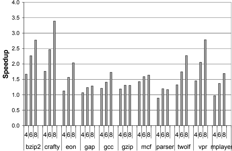
Figure 10: Speedup of Relaxed-Pure over sequential Relaxed on SPEC benchmarks while varying number of workers.
