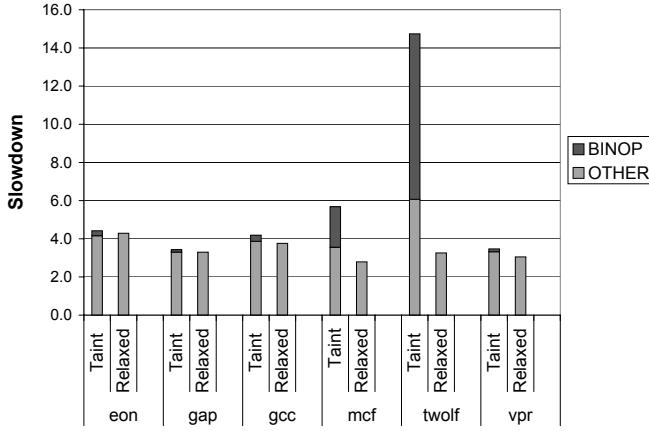
Figure 8: Application slowdown with Relaxed-Hybrid and Original-Hybrid monitoring (1 worker, 8-core configuration).
