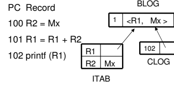
Figure 6: Simple code snippet and its summary.
