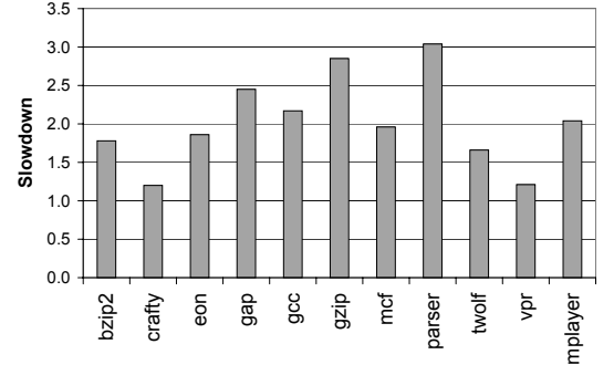
Figure 11: Application slowdown with Relaxed-Pure using 8 workers.
