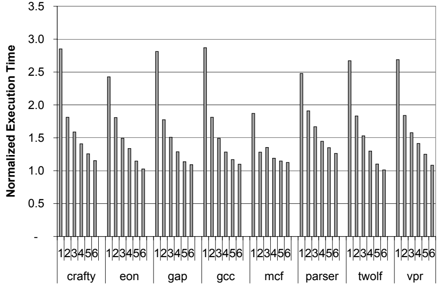
Figure 9: Execution time of Relaxed-Pure normalized to that of Relaxed-Hybrid (1 to 6 workers, 8-core configuration).
