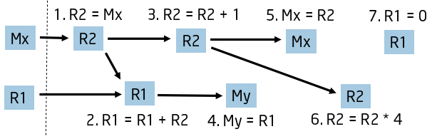
Figure 1: Example code segment, showing the information flow dependencies.
