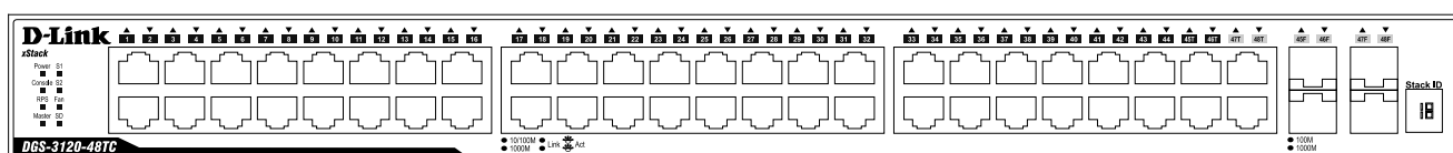
Figure 1-5 Front panel view of the DGS-3120-48TC
