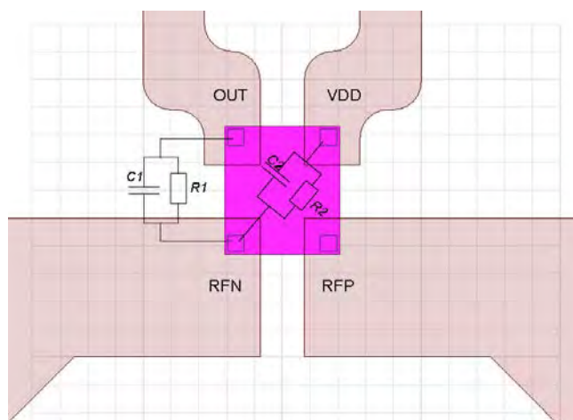
Fig 11. Model for RFID Label Antenna utilizing G2iL+ anti-tamper feature: equivalent circuitry
