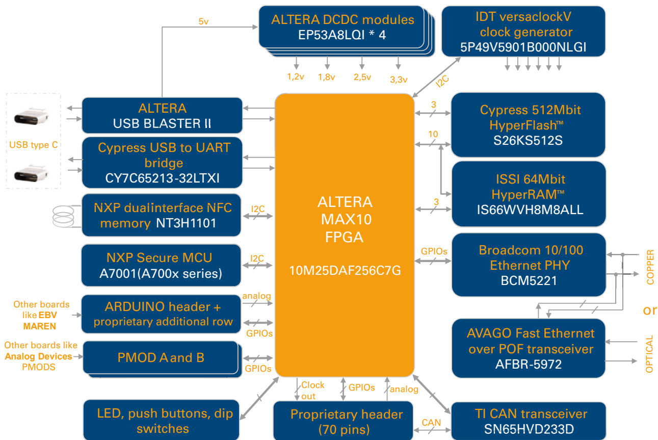
HyperMAX Block Diagram
