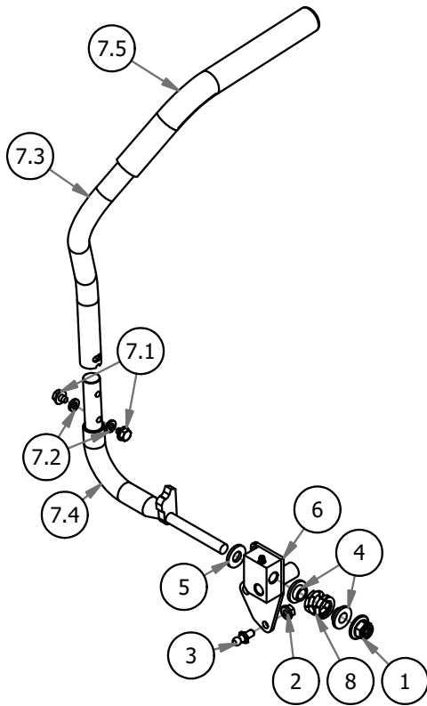
031-0017-01 ZT Steering Arm Assembly, Left Hand
