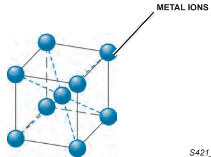
Body-Centered Cubic
