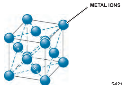
Face-Centered Cubic
