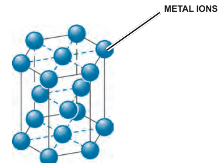
Hexagonal
