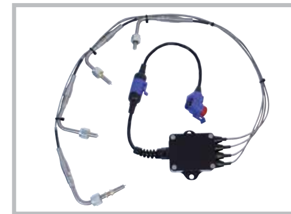
D. EXHAUST GAS TEMPERATURE JUNCTION
