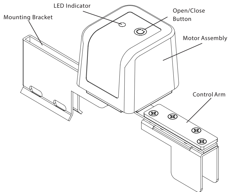
Figure 1 - Main Parts of the Water Main Shut-Off
