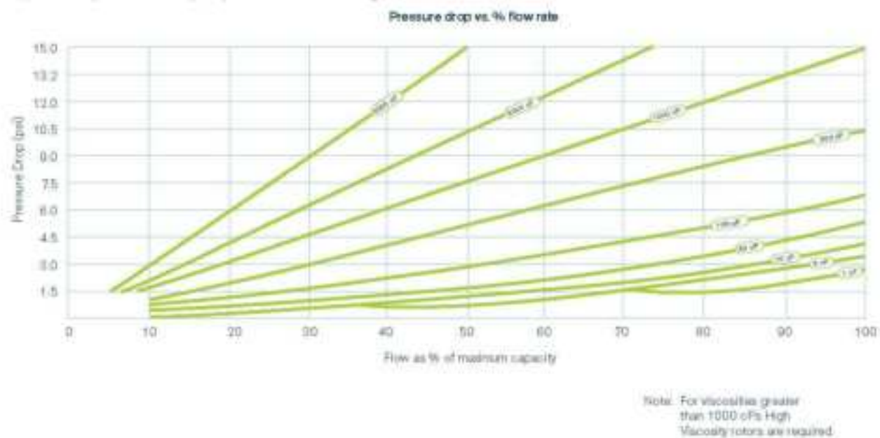
Figure 2: Impact of viscosity on pressure loss for a range of flow rates
