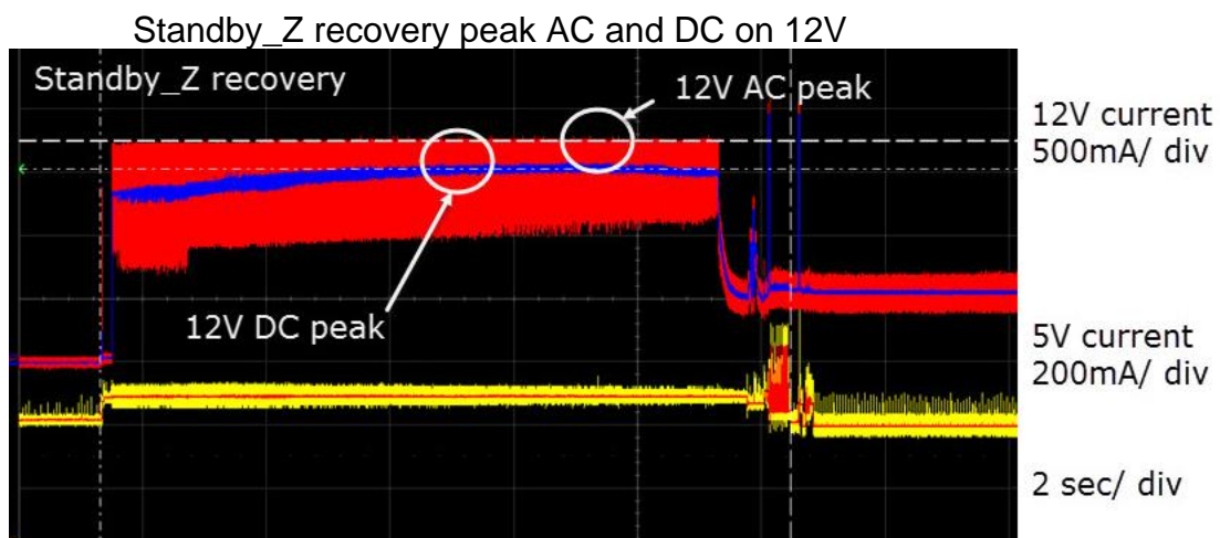
Figure 8 Standby_Z recovery current waveform
