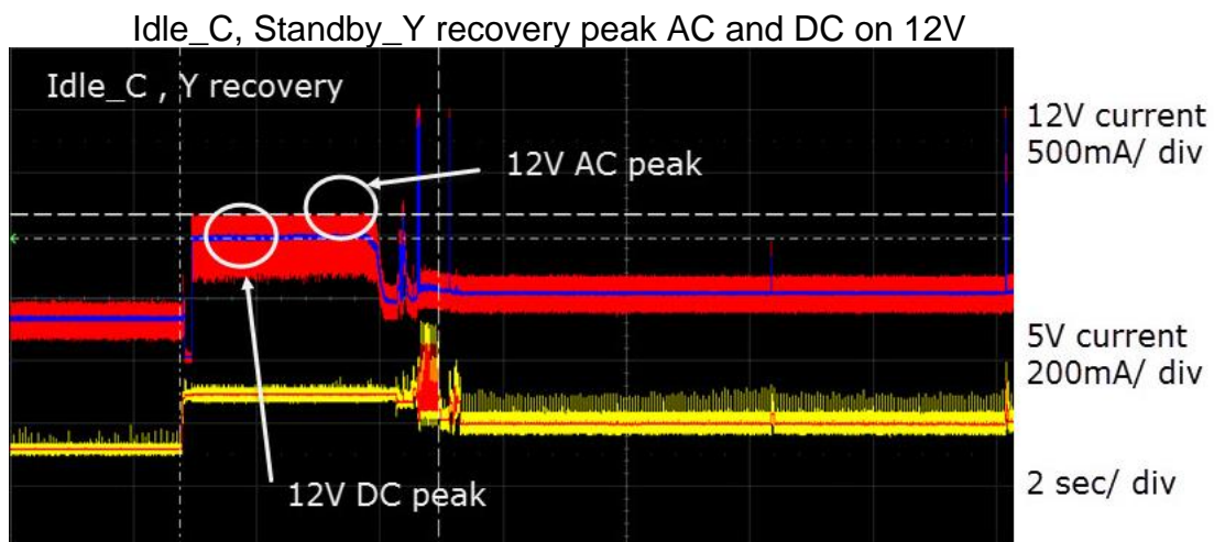
Figure 7 Idle_C Standby_Y recovery current waveform
