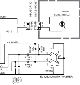
U015 Standby switch PC board BASW-0111
