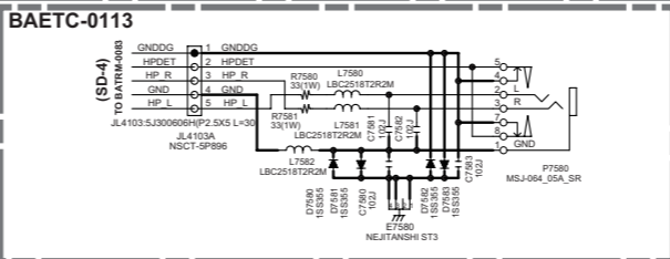
U017 Headphone terminal PC board BAETC-0113
