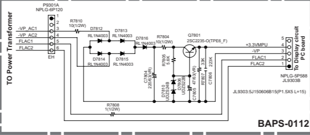
U016 FL Power supply PC board BAPS-0112
