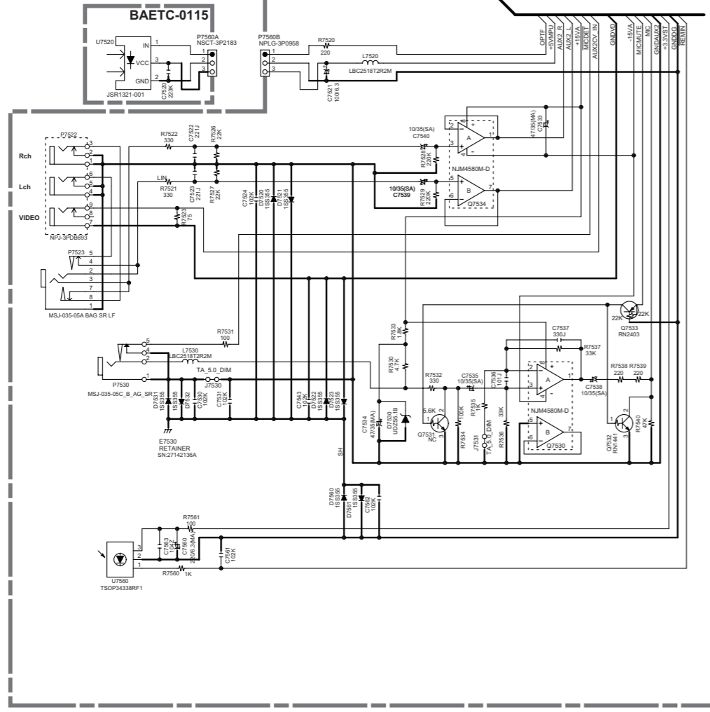
U019 AUX Input terminal PC board BAETC-0115
