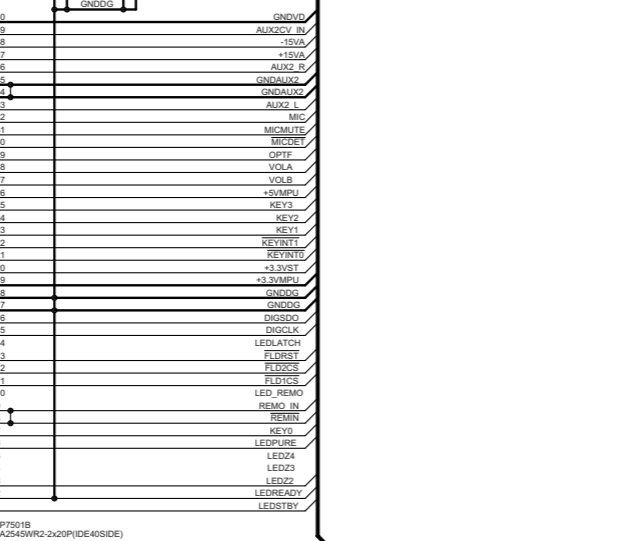
U019 AUX Input terminal PC board BAETC-0115
