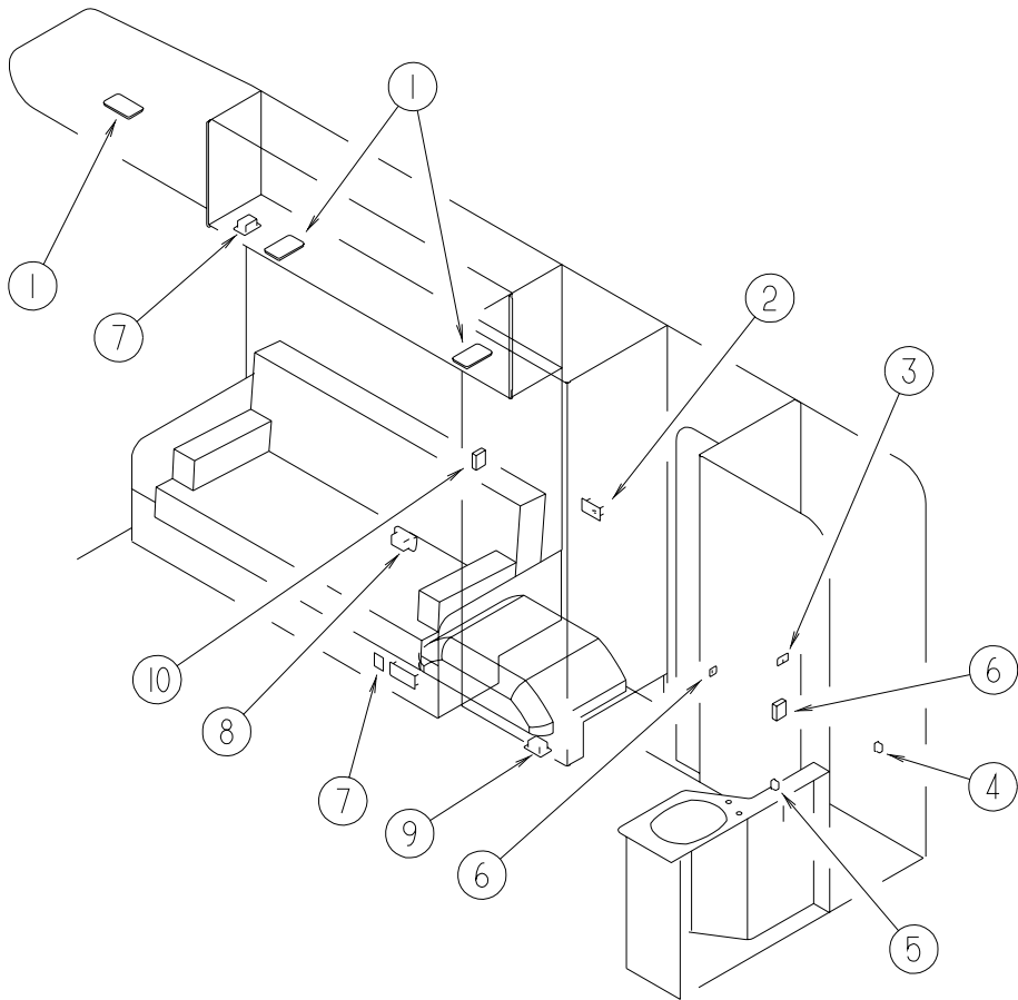
LIGHTS, SWITCHES & RECEPTACLES - PASSENGER SIDE
