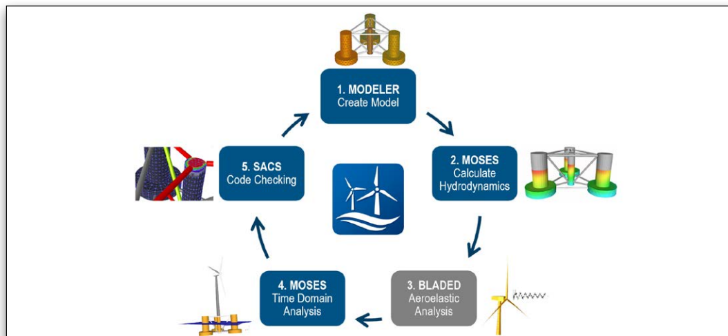
OpenWindPower Floating Platform workflow.
