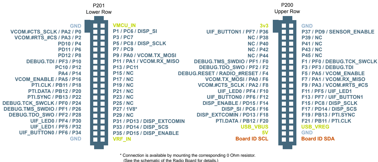
Figure 2.1. BRD4305E Radio Board Connector Pin Mapping
