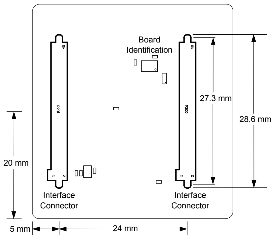
Figure 4.2. BRD4305E Bottom View
