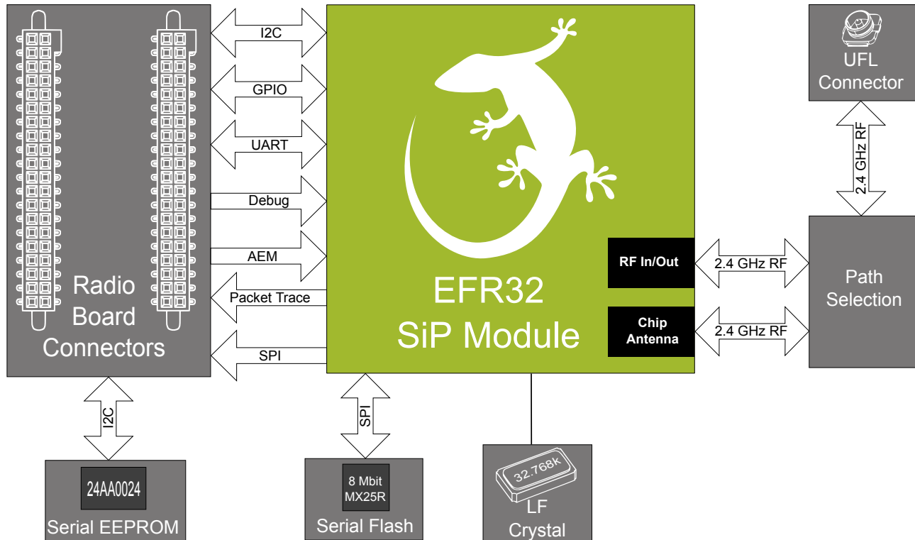
Figure 3.1. BRD4305E Block Diagram
