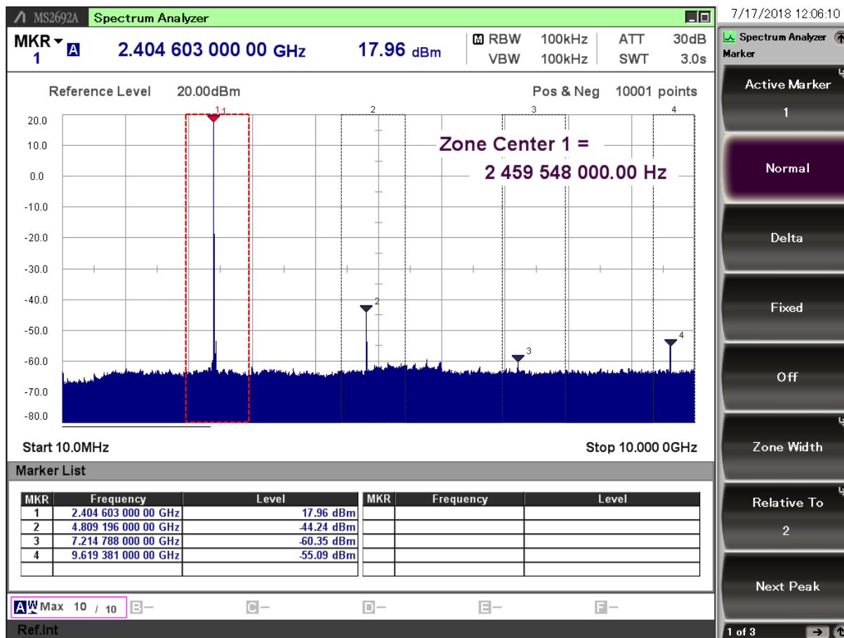
Figure 6.1. Typical Output Spectrum of the BRD4305E
