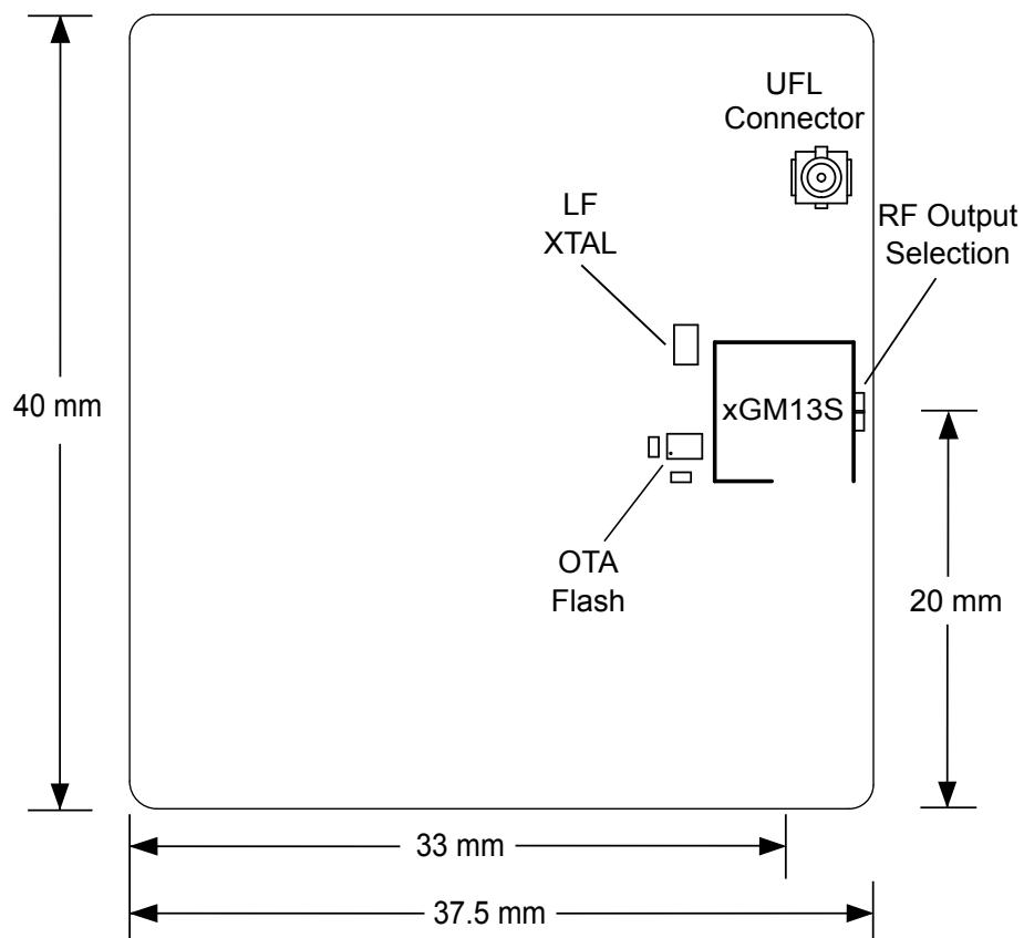
Figure 4.1. BRD4305E Top View
