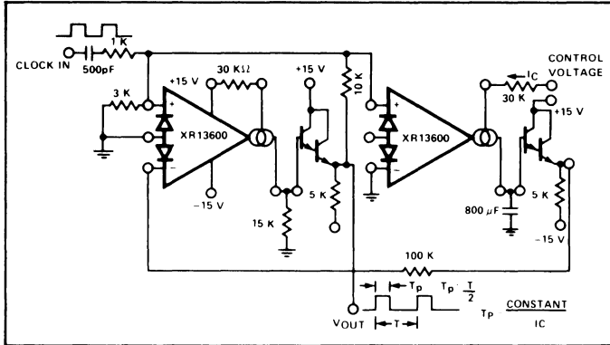
Figure 30. Pulse Width Modulator
