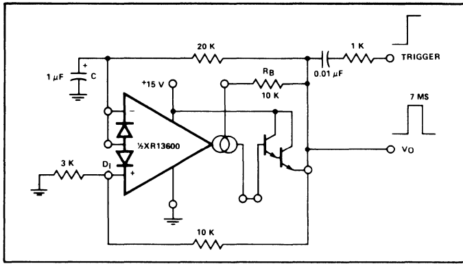
Figure 19. Timer With Zero Stand-By Power
