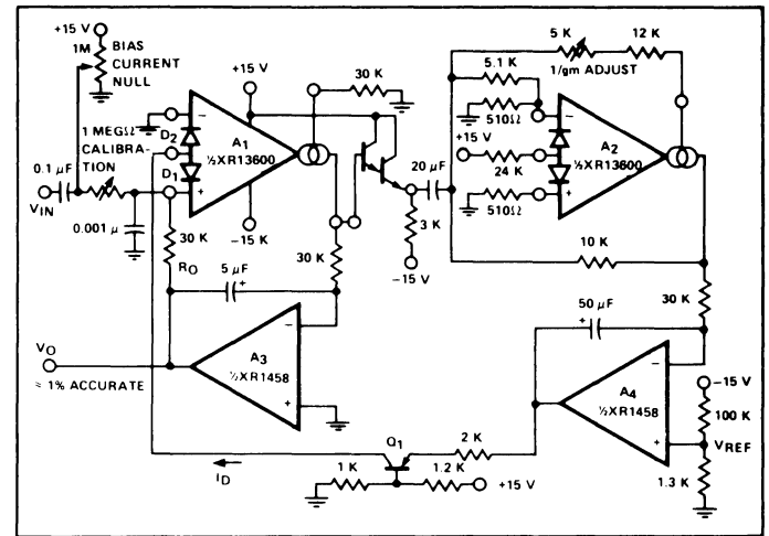
Figure 27. True RMS Converter Circuit
