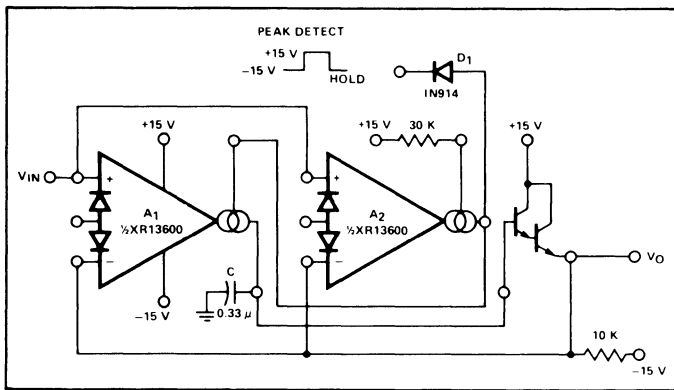
Figure 25. Peak Detector and Hold Circuit
