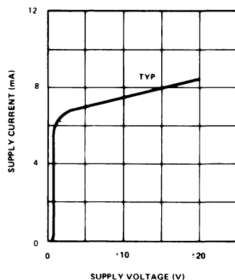
SUPPLY CURRENT
