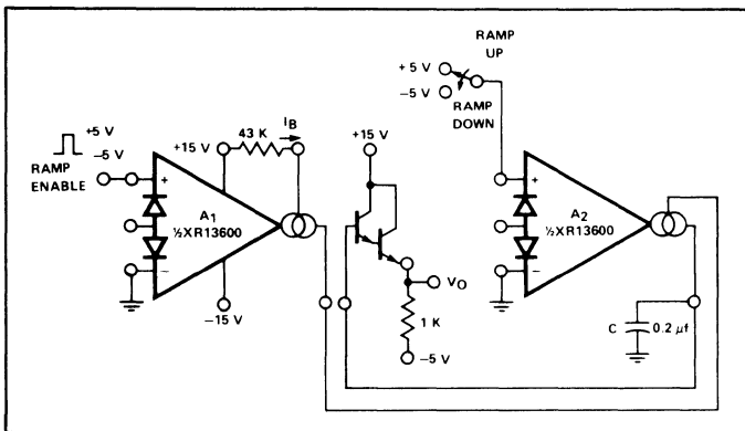
Figure 26. Ramp and Hold Circuit
