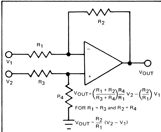
Figure 5. Difference Amplifier
