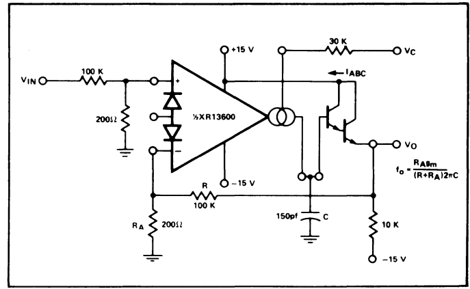
Figure 11. Voltage Controlled Low-Pass Filter
