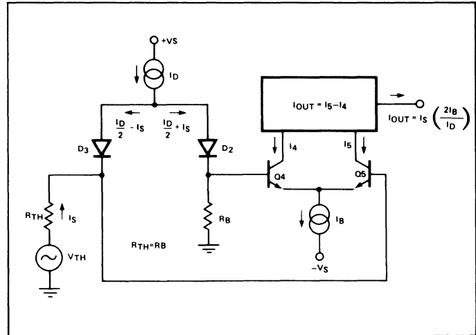
Figure 3. Equivalent VCA Input Circuit
