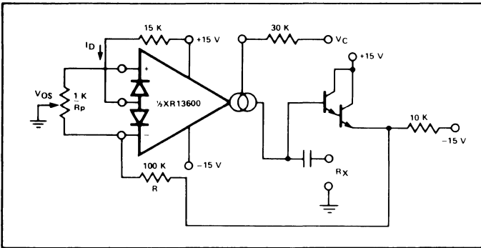
Figure 9. Voltage Controlled Resistor with Linearizing Diodes
