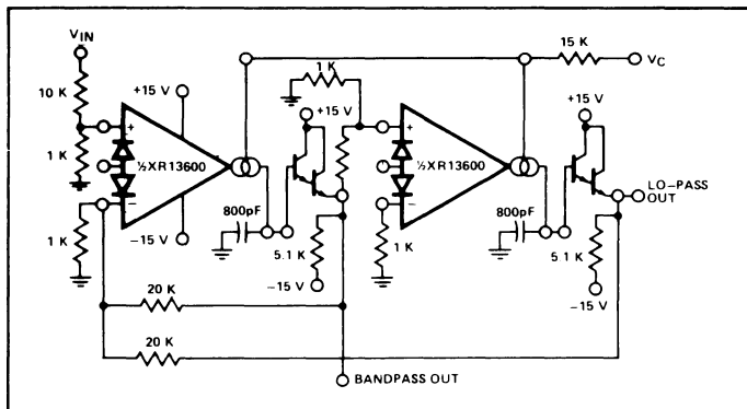
Figure 14. Voltage Controlled State Variable Filter
