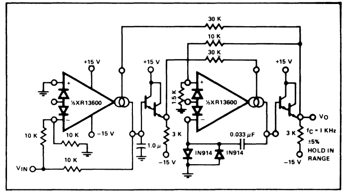
Figure 21. Phase-Locked Loop
