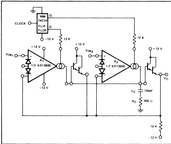
Figure 20. Multiplexer
