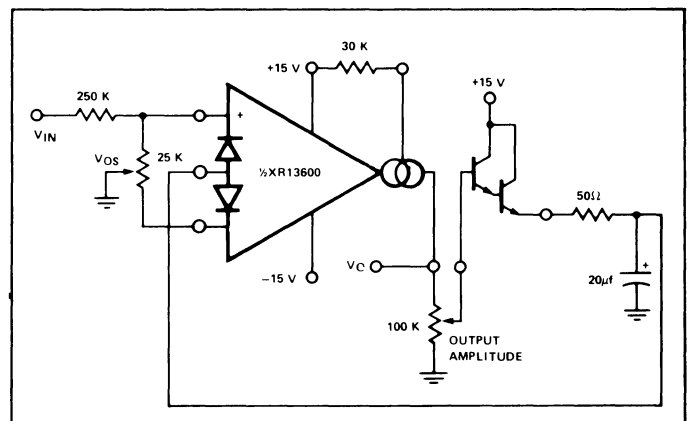
Figure 7. AGC Amplifier
