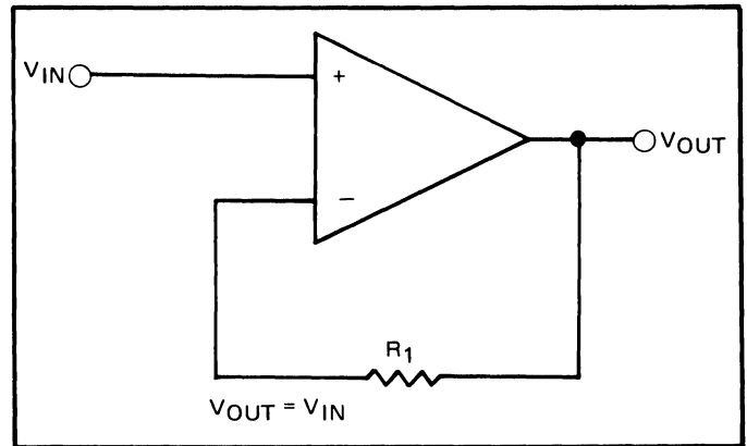
Figure 3. Unity-Gain Buffer
