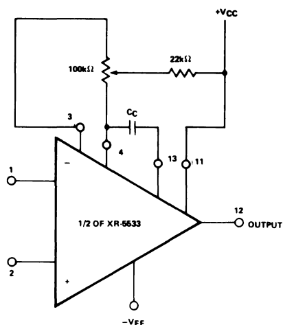
FREQUENCY COMPENSATION AND OFFSET VOLTAGE ADJUSTMENT CIRCUIT
