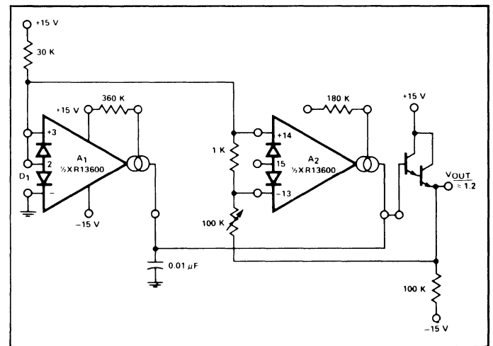
Figure 28. Delta V_{BE} Reference
