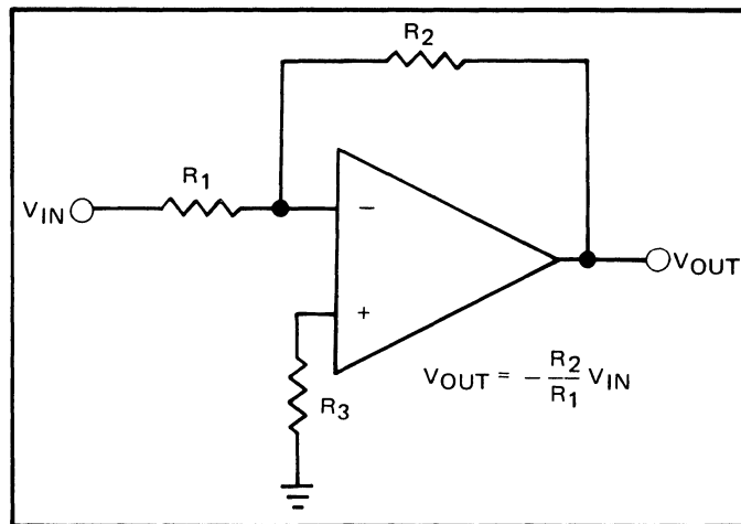
Figure 1. Inverting Amplifier
