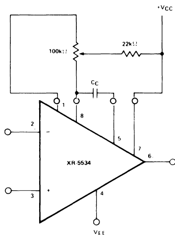
FREQUENCY COMPENSATION AND OFFSET VOLTAGE ADJUSTMENT CIRCUIT
