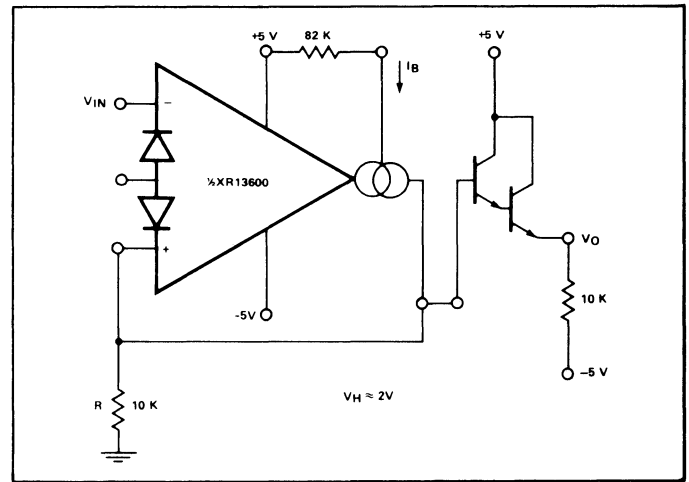
Figure 22. Schmitt Trigger
