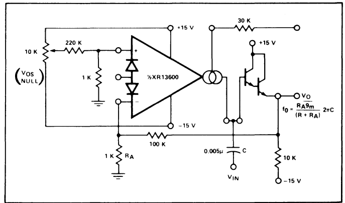
Figure 12. Voltage Controlled High-Pass Filter
