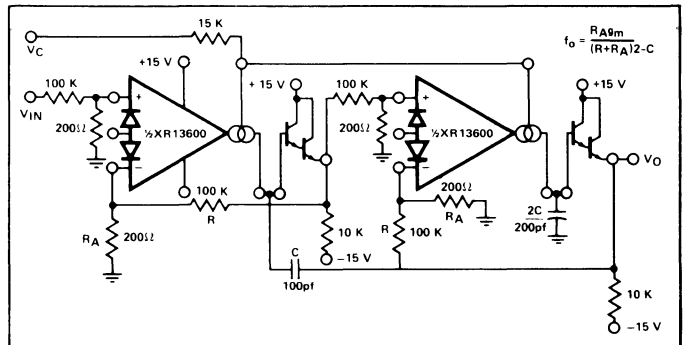
Figure 13. Voltage Controlled 2-Pole Butterworth Low-Pass Filter
