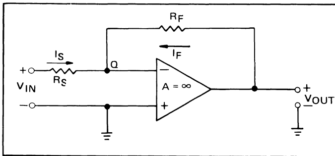
Figure 1. The “Ideal” Operational Amplifier as a Feedback Amplifier.
