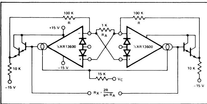
Figure 10. Floating Voltage Controlled Resistor
