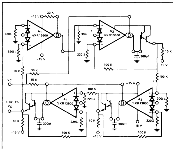
Figure 17. Sinusoidal VCO using two XR-13600 Circuits
