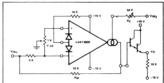
Figure 6. Four-Quadrant Multiplier
