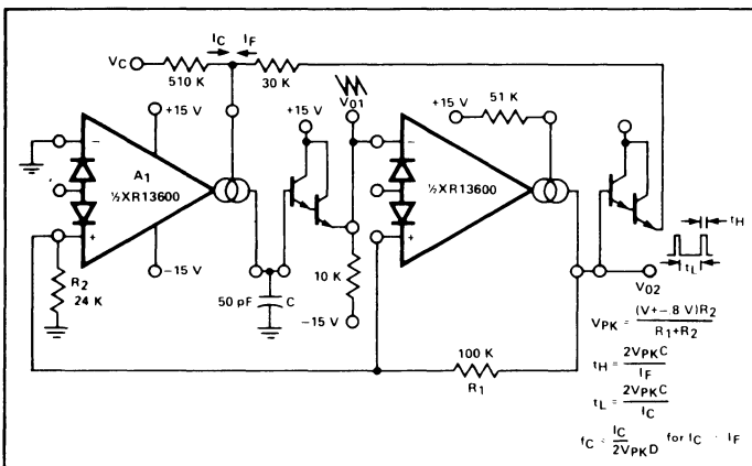
Figure 16. Ramp/Pulse VCO
