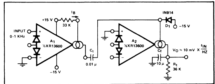
Figure 23. Tachometer
