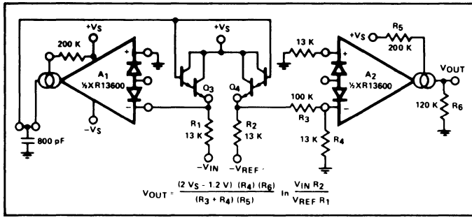
Figure 29. Log Amplifier
