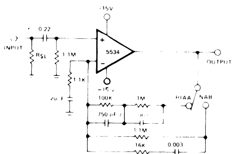
PREAMPLIFIER-RIAA/NAB COMPENSATION
