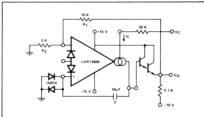
Figure 18. Single Amplifier VCO
