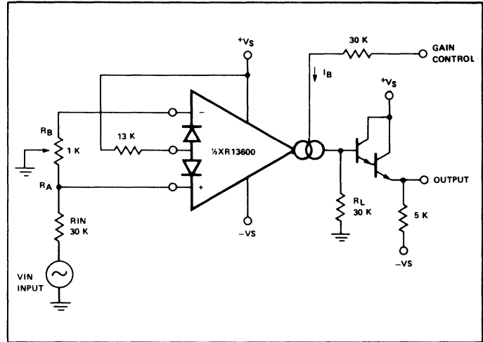
Figure 2. Voltage Controlled Amplifier (VCA) Circuit
