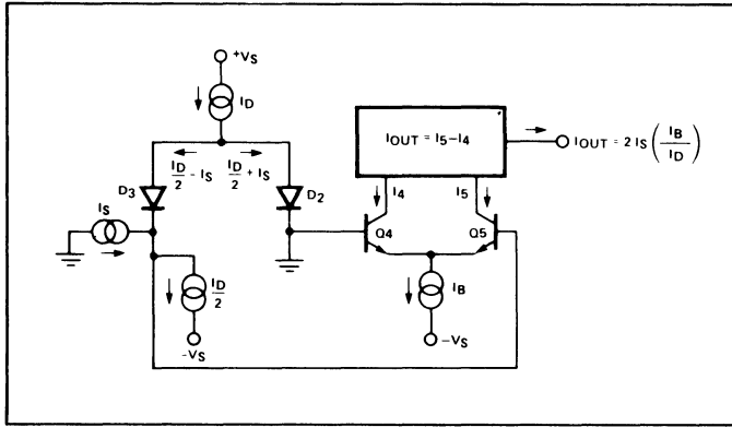
Figure 1. Linearizing Diodes
