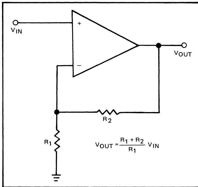
Figure 2. Non-Inverting Amplifier
