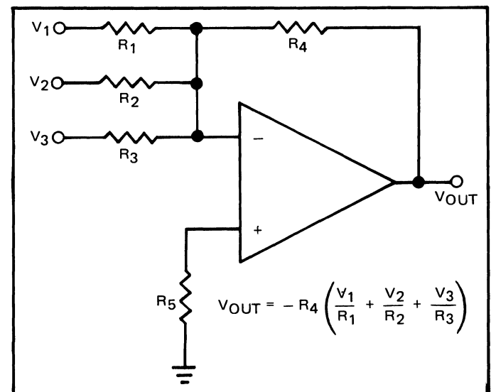
Figure 4. Summing Amplifier
