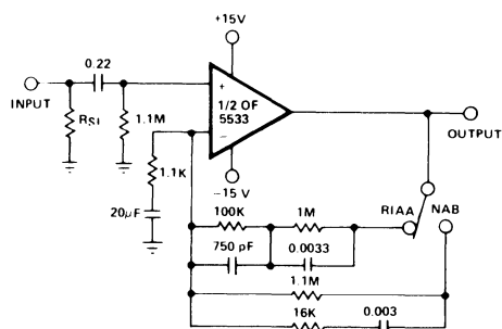
PREAMPLIFIER—RIAA/NAB COMPENSATION
