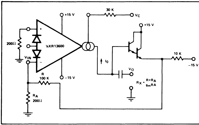
Figure 8. Voltage Controlled Resistor, Single-Ended
