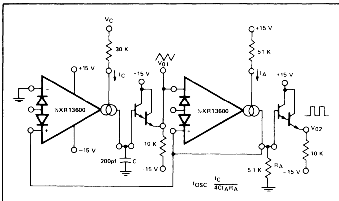
Figure 15. Triangular/Square-Wave VCO
