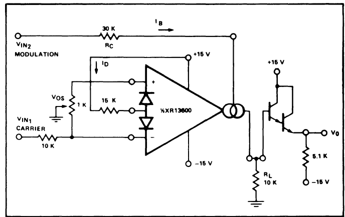
Figure 5. Amplitude Modulator
