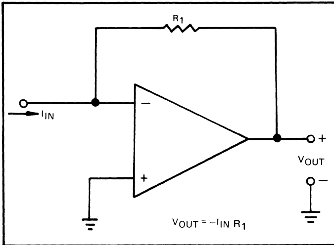
Figure 11. Operational Amplifier as a Current-to-Voltage Converter.
