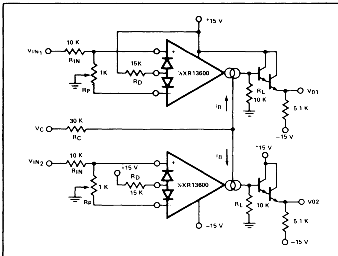
Figure 4. Stereo Volume Control
