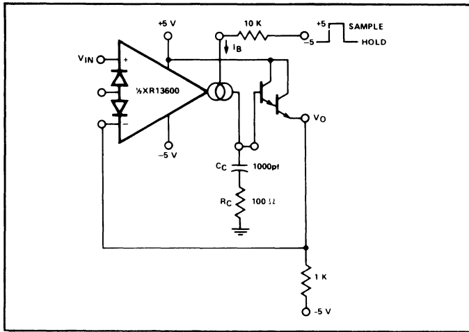
Figure 24. Sample-and-Hold Circuit
