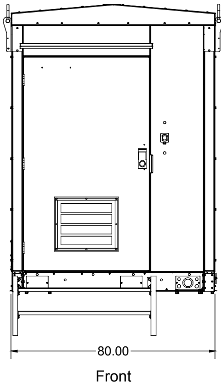
Figure 2-3: Overall Dimensions
