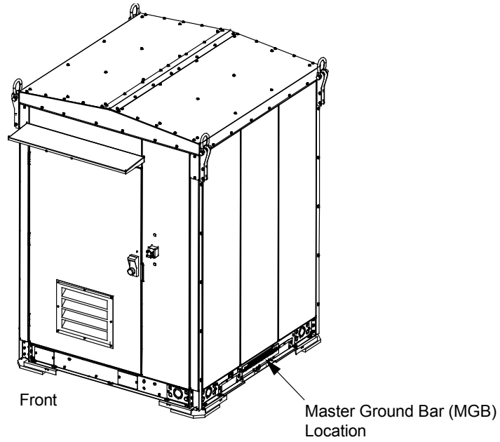
Figure 9-1: XTE 802G Master Ground Bar (MGB) Location
