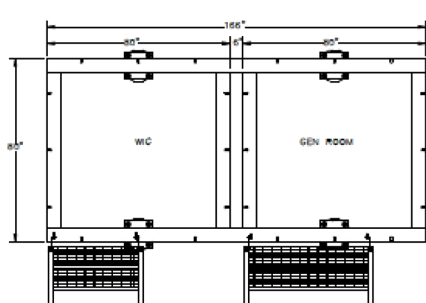
Figure 6-6: XTE 802 and XTE 802G Combo Helical Platform
