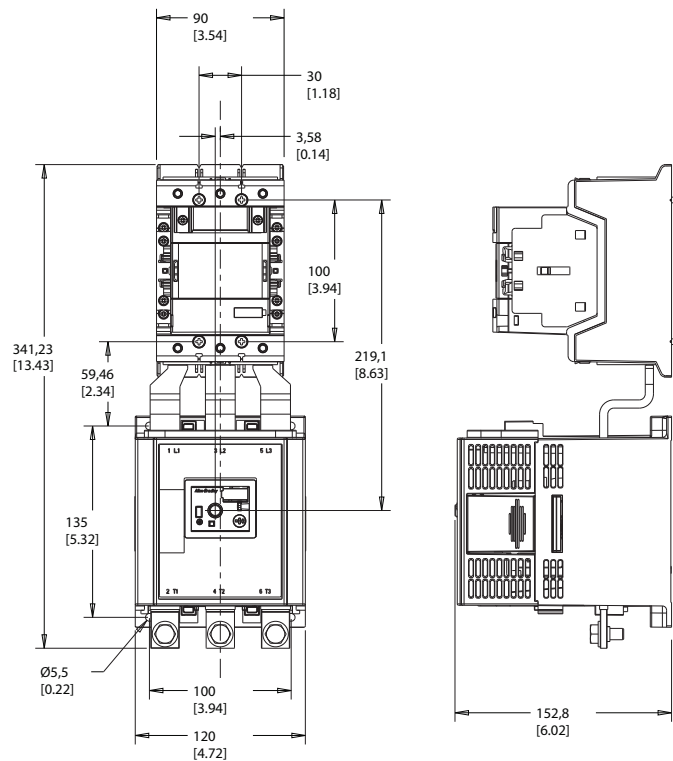
Figure 12 - E1 Plus with Bulletin 100-E116 and 100-E146 Contactors
