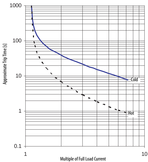
Figure 4 - Trip Class 10
