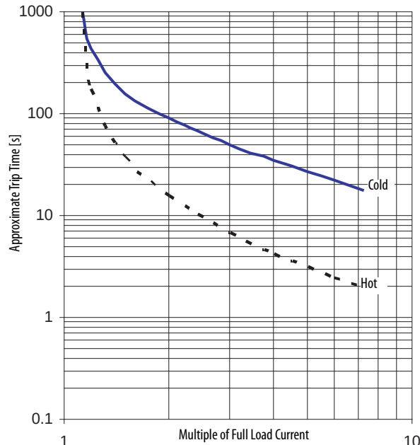
Figure 7 - Trip Class 30
