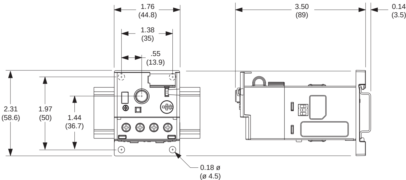
Figure 8 - E1 Plus Pass-thru Style
