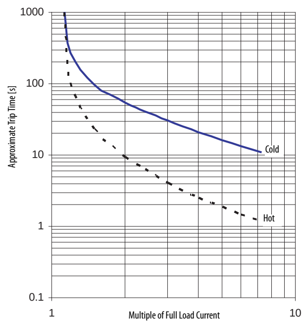
Figure 5 - Trip Class 15
