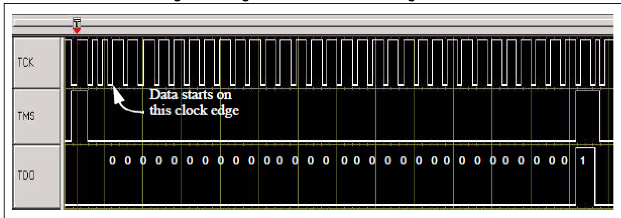
Figure 12. Signal transitions for reading DBCR0
