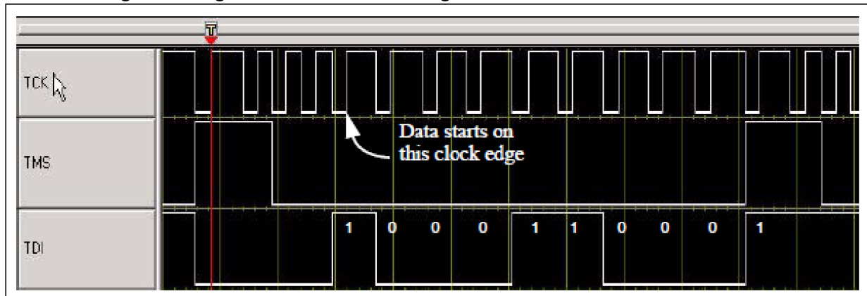
Figure 11. Signal transitions for writing OCMD to select a read from DBCR0
