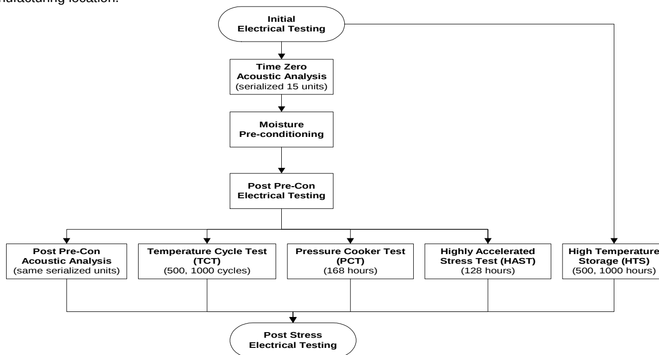
Figure 1. Cypress Package Reliability Stress Flow
