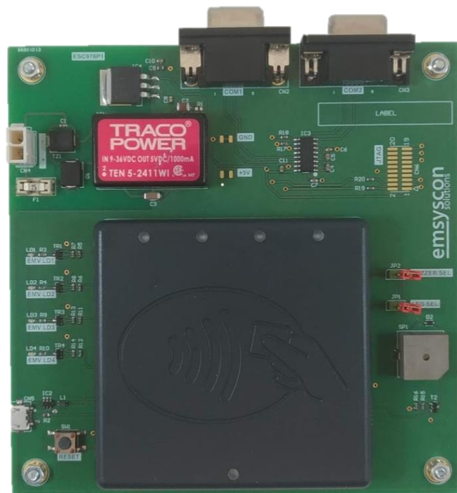
Figure 6: Connection via 16-way connector
