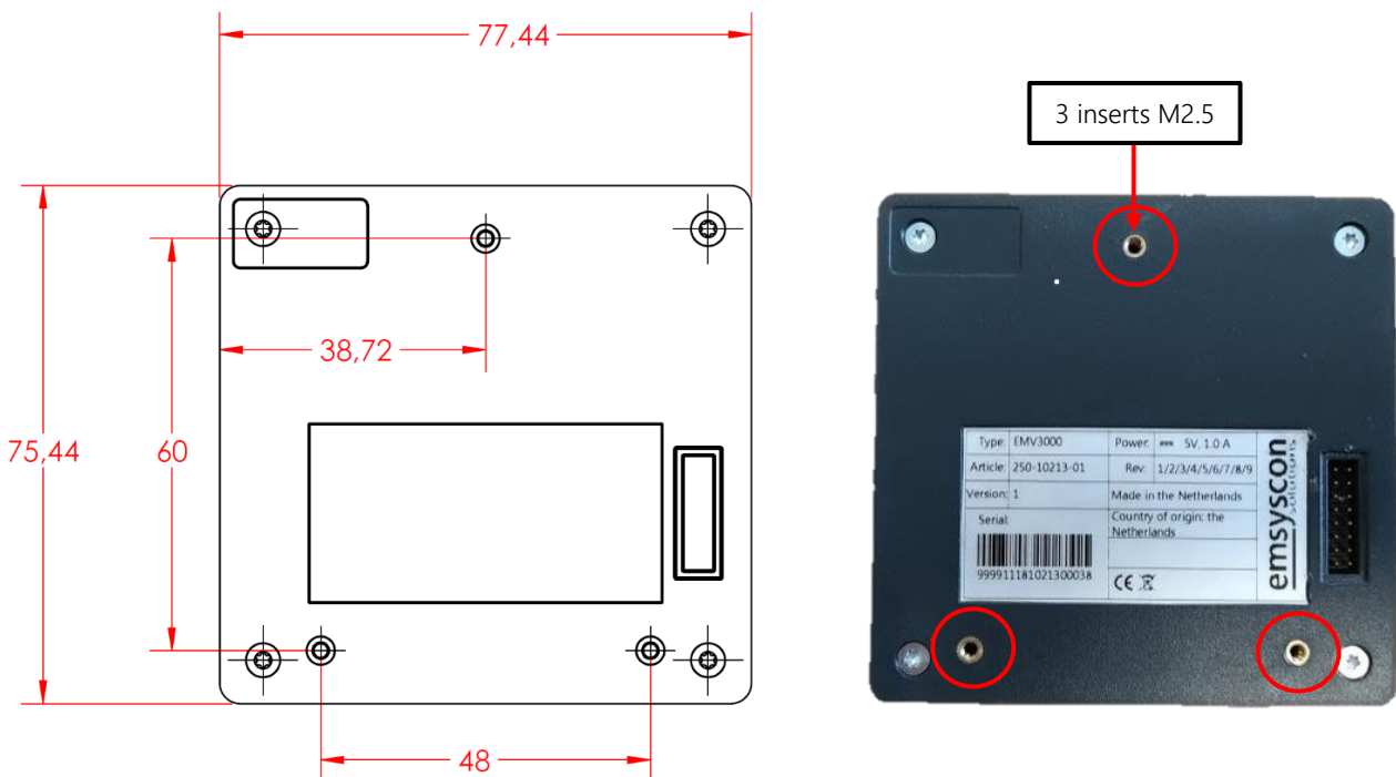
Figure 3: Mounting holes
