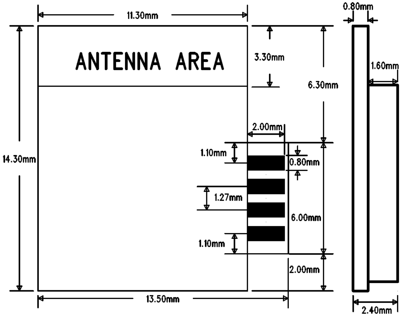
Fig 2 Top View Module Size
