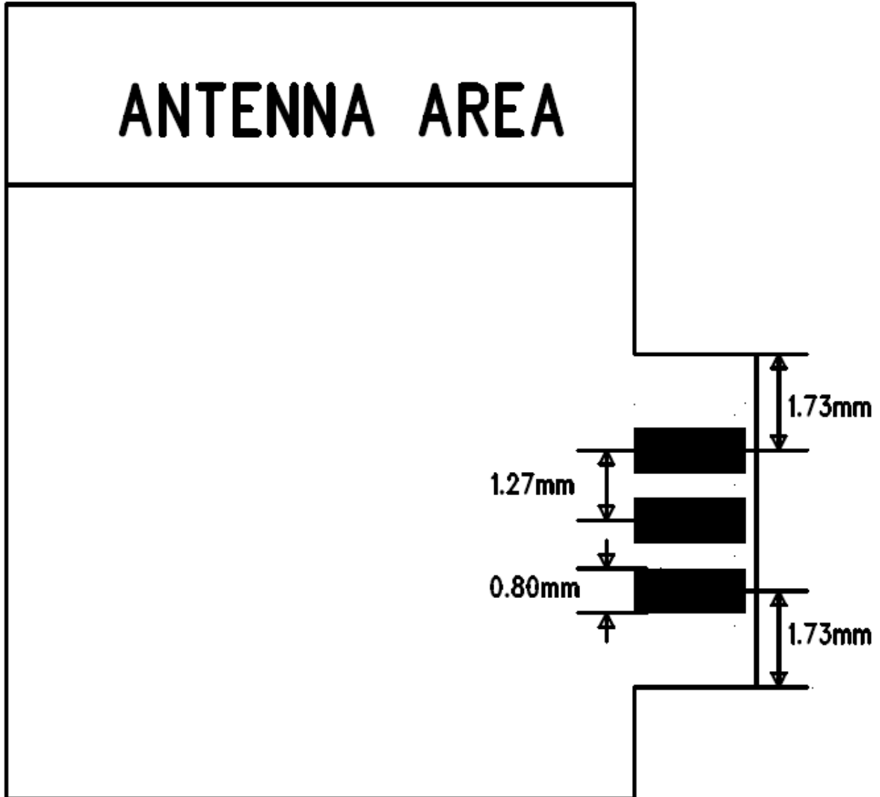
Fig 3 EWN-8258FAT1HA Bottom View Module Size
