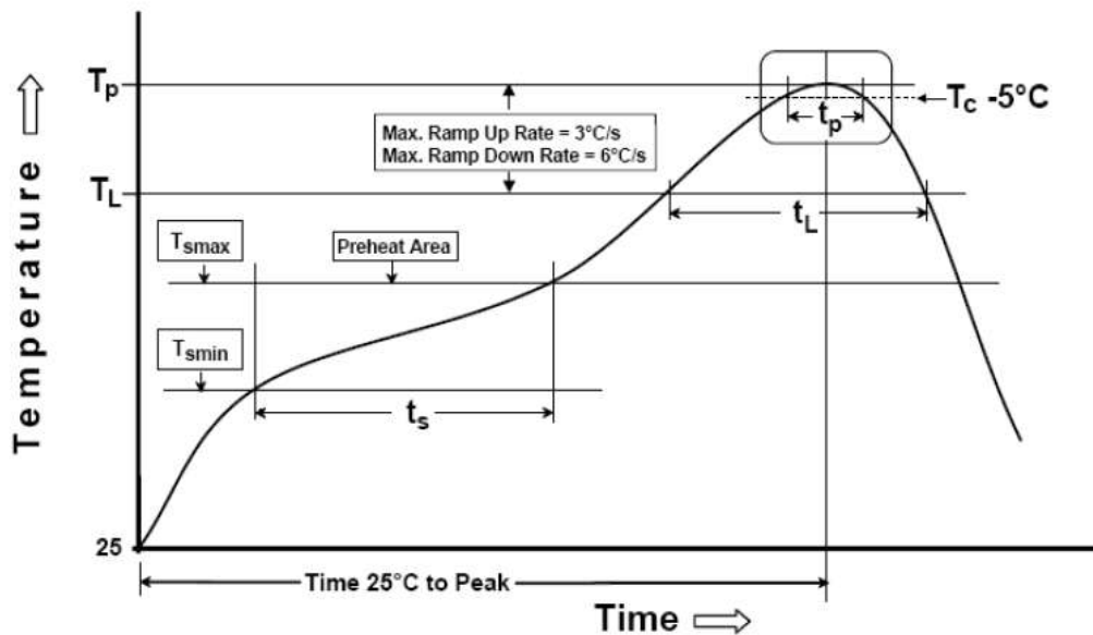
Fig 13 Furnace temperature curve
