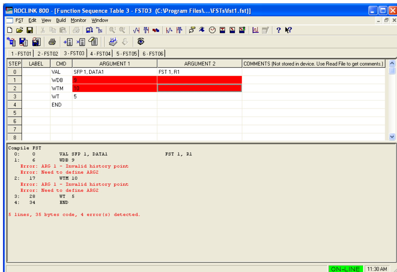
Figure 2-8. Compile Errors
