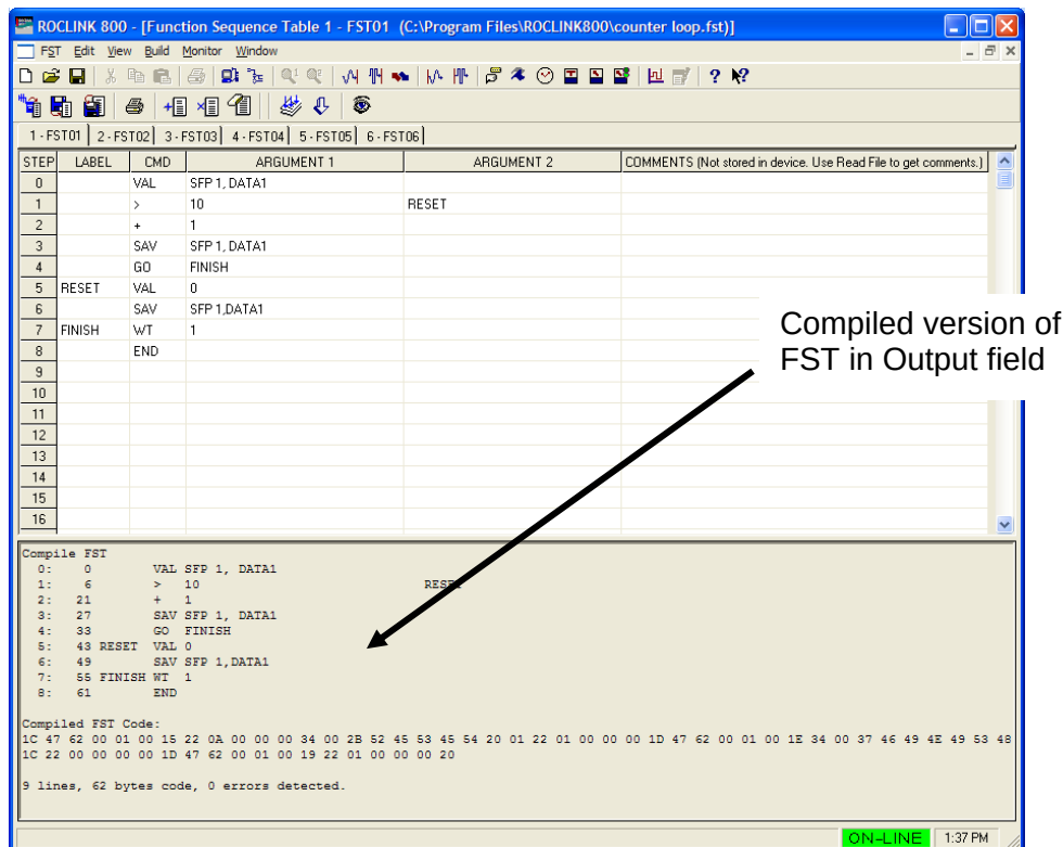
Figure 2-3. Compiled FST
