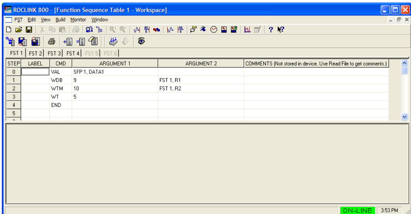
Figure 4-5 Sample FST
