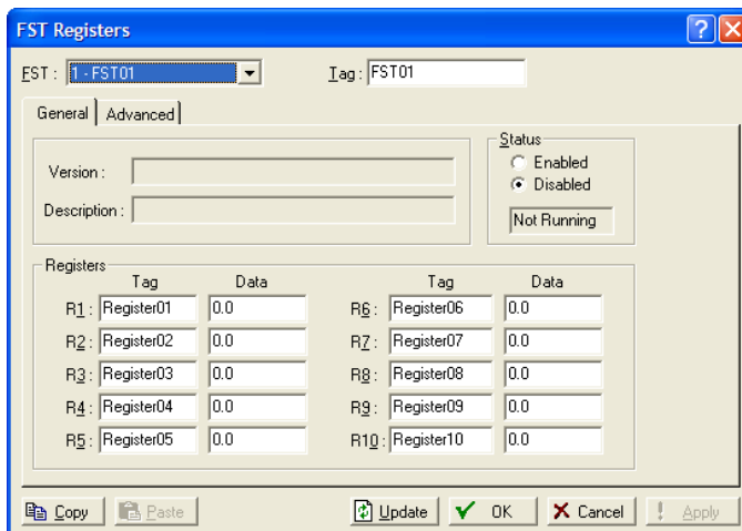
Figure 1-3. FST Registers, General tab (ROC800-Series)
