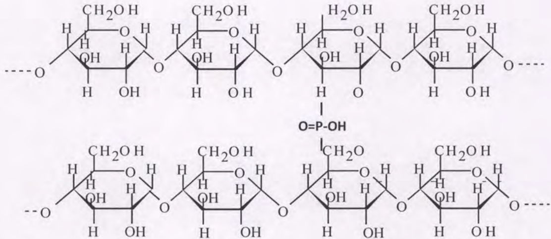
Figure 2. Structural Formula for Distarch Phosphate
