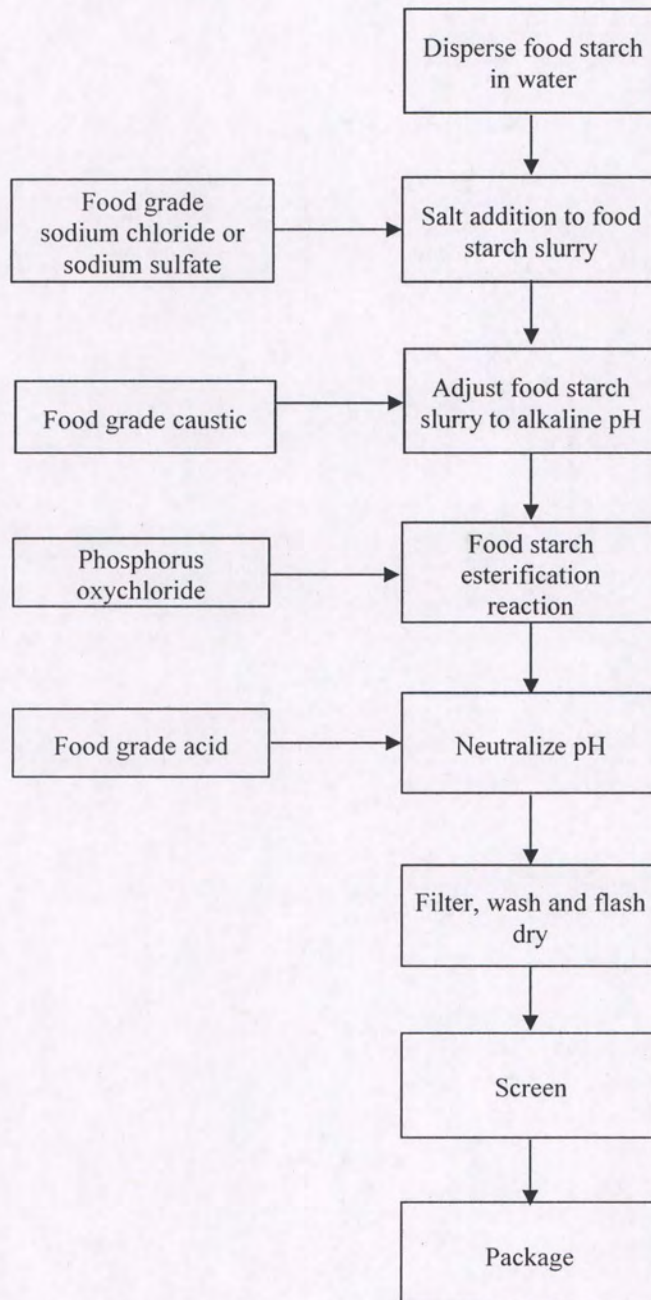
Figure 3. Distarch Phosphate Process Flow Diagram
