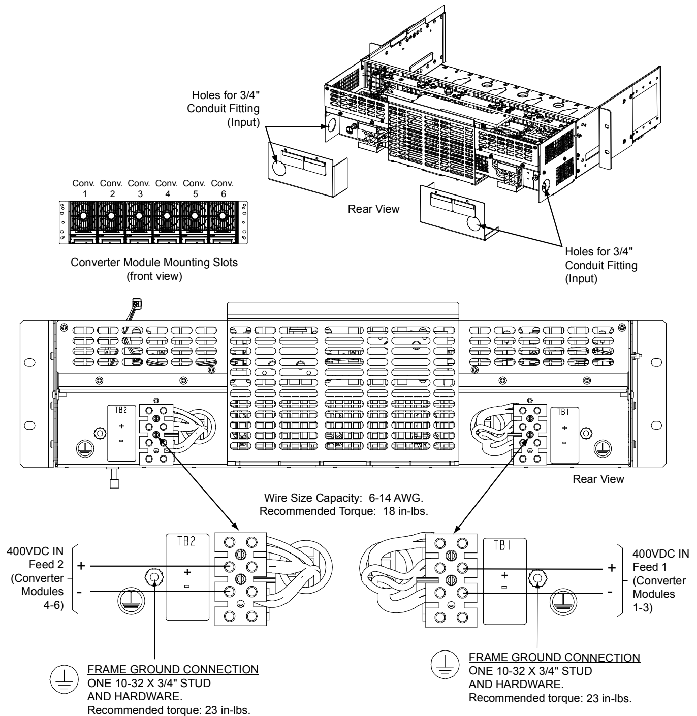
CONVERTER 400VDC INPUT FEEDS 1 FEED PER 3 CONVERTERS
