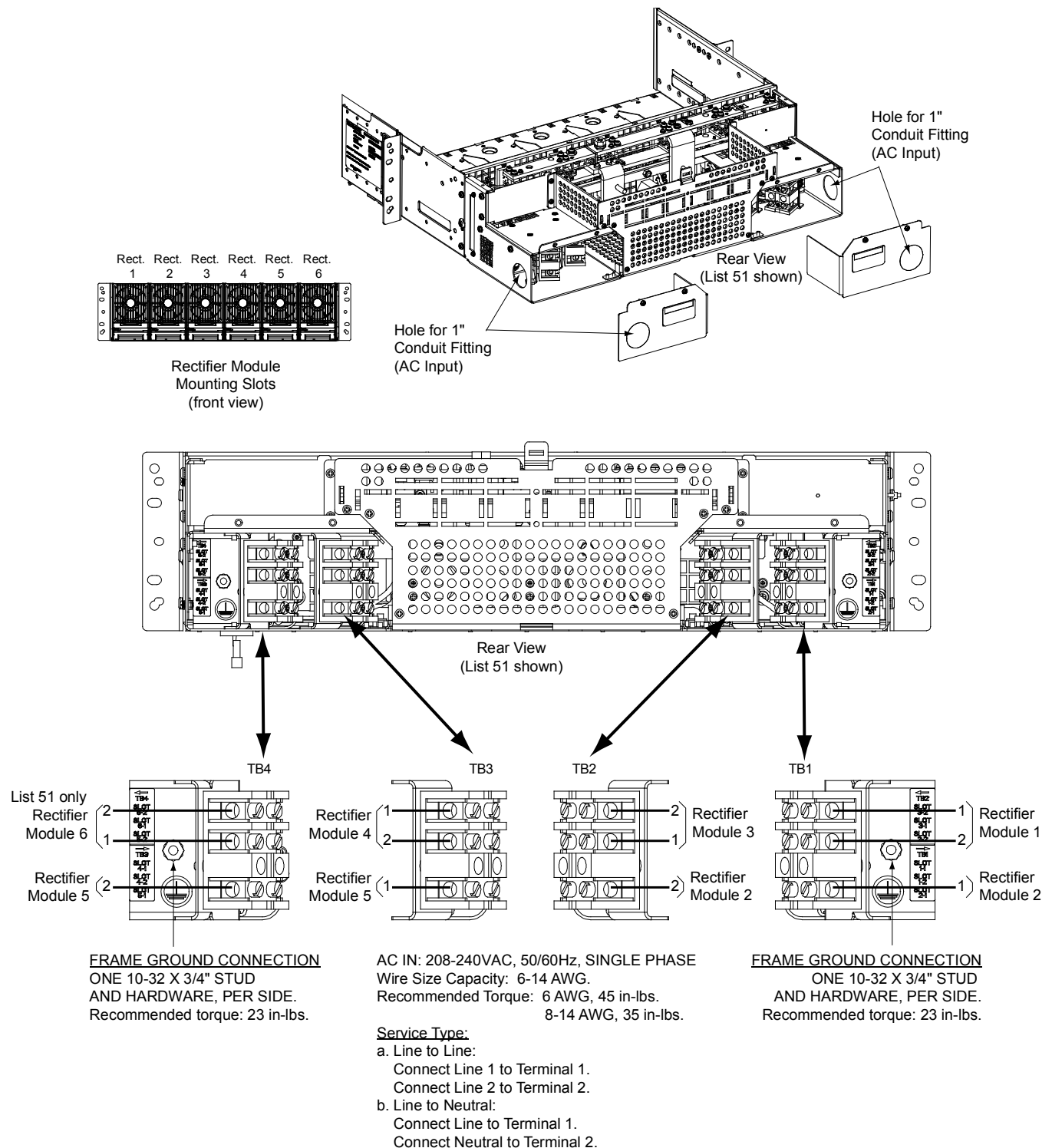
Figure 2 List 51 and 61 AC Input and Frame Ground Connections (Single-Phase Input) (Terminal Blocks)
