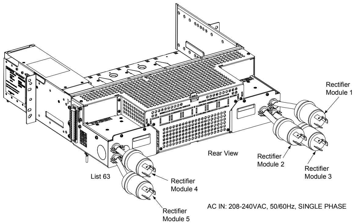
Figure 7 List 53 and 63 AC Input Connections (Single-Phase Input) (Line Cords)
