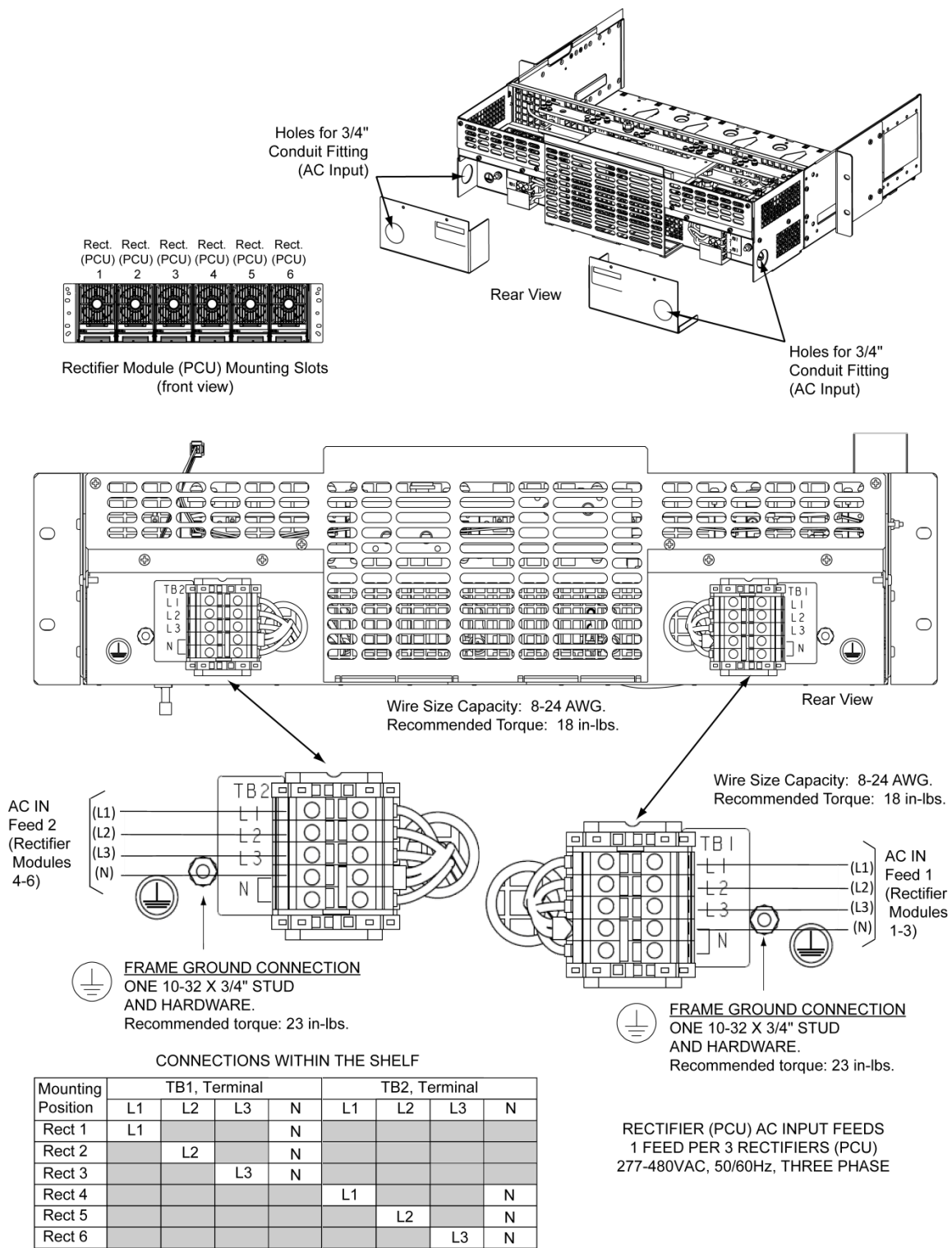
Figure 4 List 33 AC Input and Frame Ground Connections (Three-Phase Input) (Terminal Blocks)
