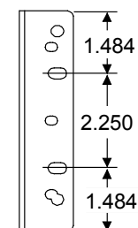
Mounting Angle Detail
