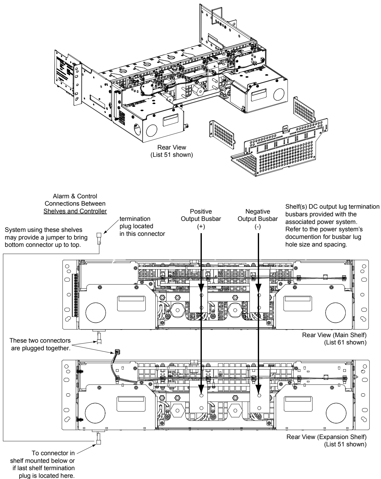
Figure 11 DC Output and Alarm/Control Connections (List 51, 52, 53, 61, 62, 63)
