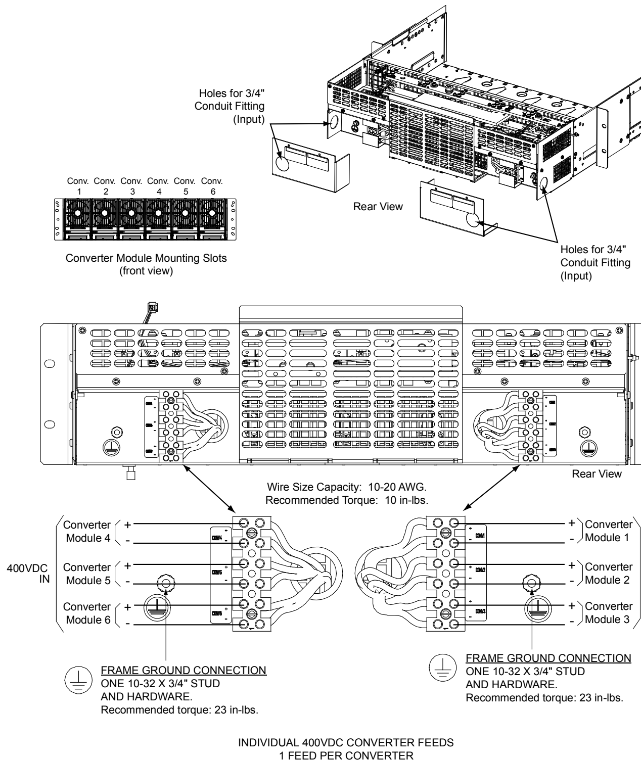
Figure 8 List 41 DC Input and Frame Ground Connections (Terminal Blocks)
