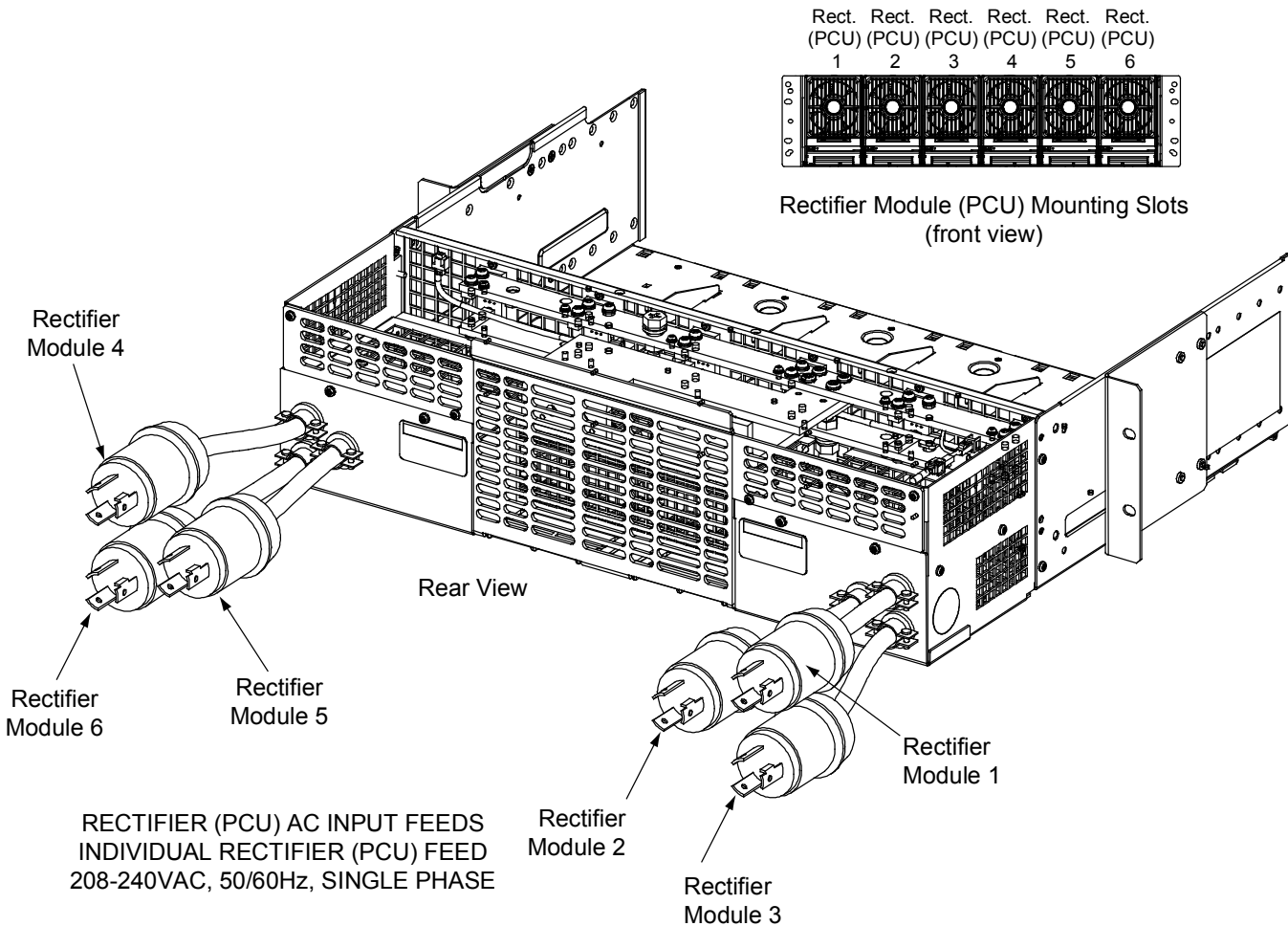
Figure 6 List 11 and 22 AC Input Connections (Single-Phase Input) (Line Cords)
