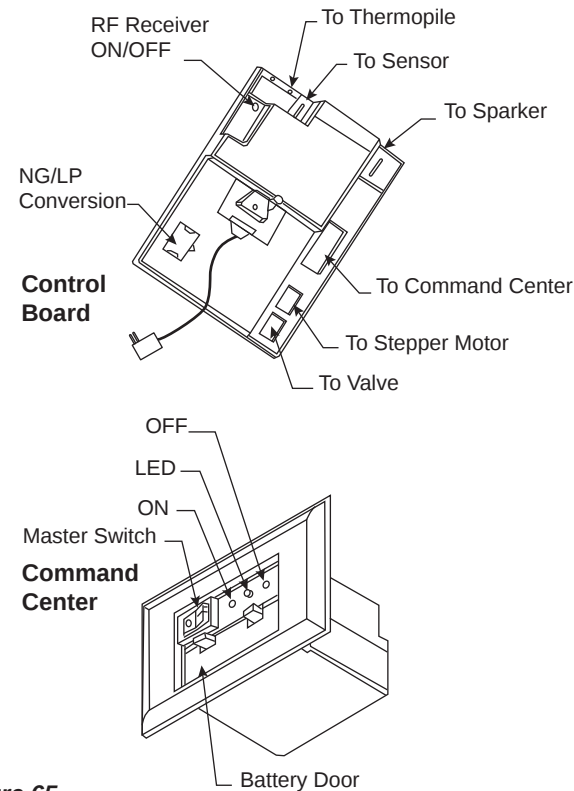
Figure 65 - Signature Command System Components
