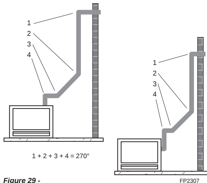
Figure 29 - Maximum Elbow Usage
