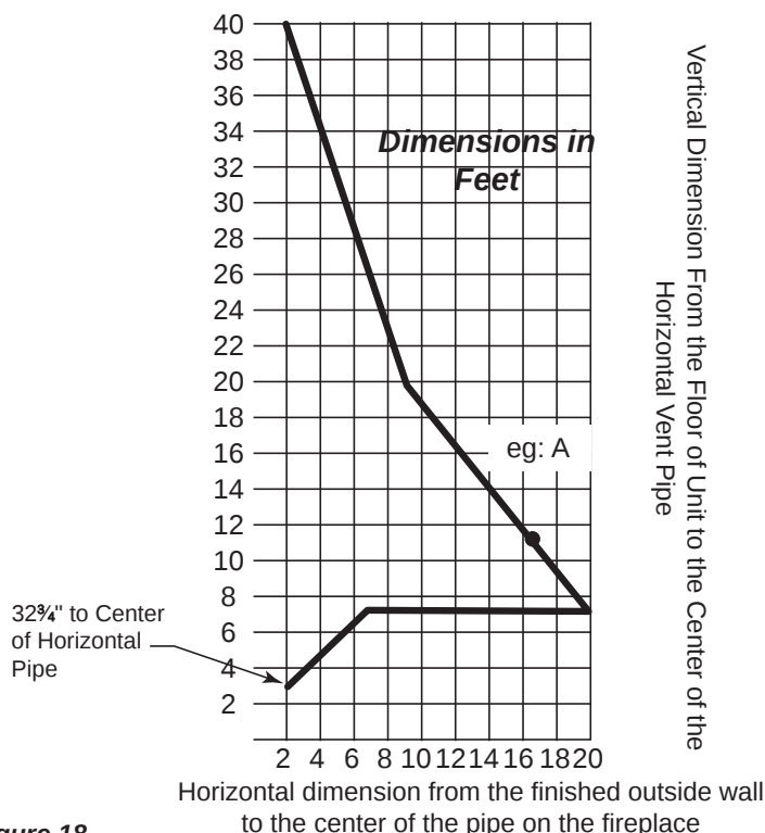
Figure 18 - Rear Wall Venting Graph
