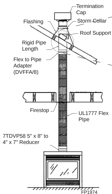
Figure 47 - Typical Vertical Flex Vent Installation
