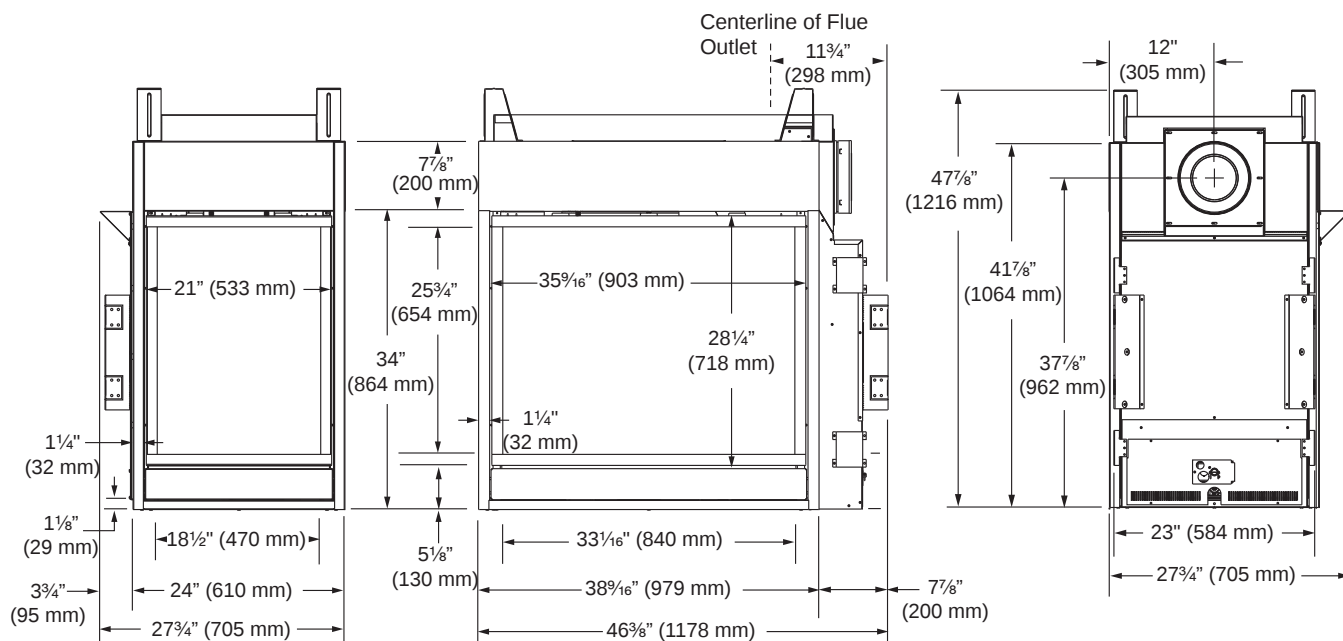
Figure 2 - STL DV (See-thru) Fireplace Dimensions
