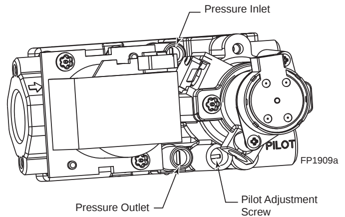
Figure 52 - Signature Command Valve
