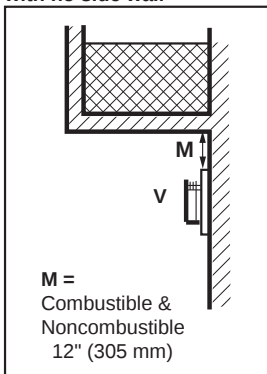
Figure 17 - Termination Clearances
