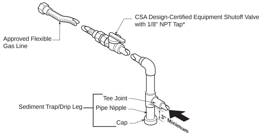
Figure 51 - Gas Connection
