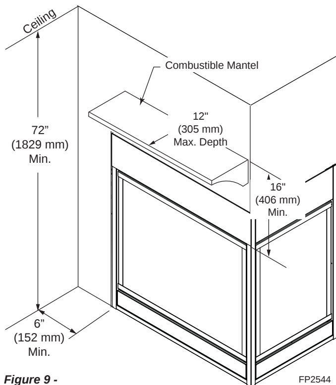
Figure 9 - Ceiling and Side Wall Clearances
