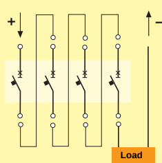
Diagram F: breaking with 4 poles in series for one polarity
