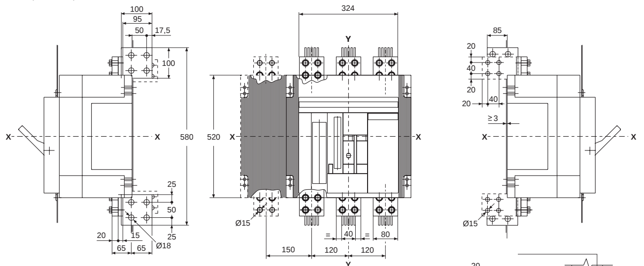
Rear (S8 3200)
