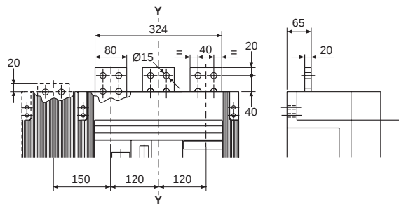
Front (S8 2000-2500)
