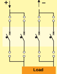
Diagram D: breaking with 2 poles in parallel per polarity
