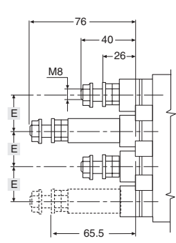
View A
