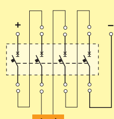
Diagram H: 2+2 poles in series
