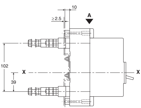
Threaded rear
