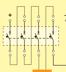
Diagram G: 3+1 poles in series
