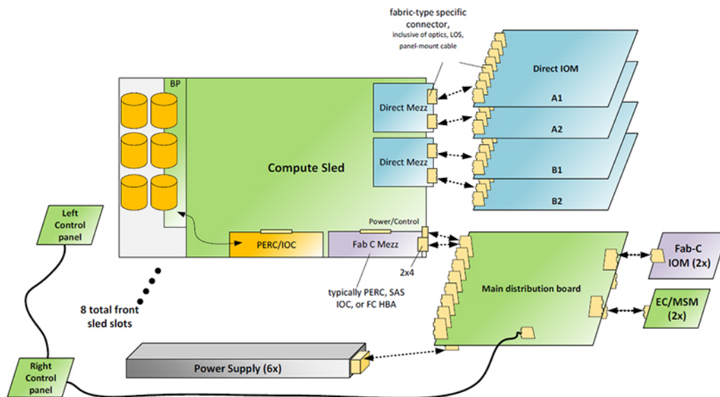
Figure 6. Internal Architecture
